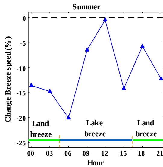
Figure S2. Changes in the hourly speed of local lake and land breezes at Urmia meteorological station in the periods with normal and low lake level.
