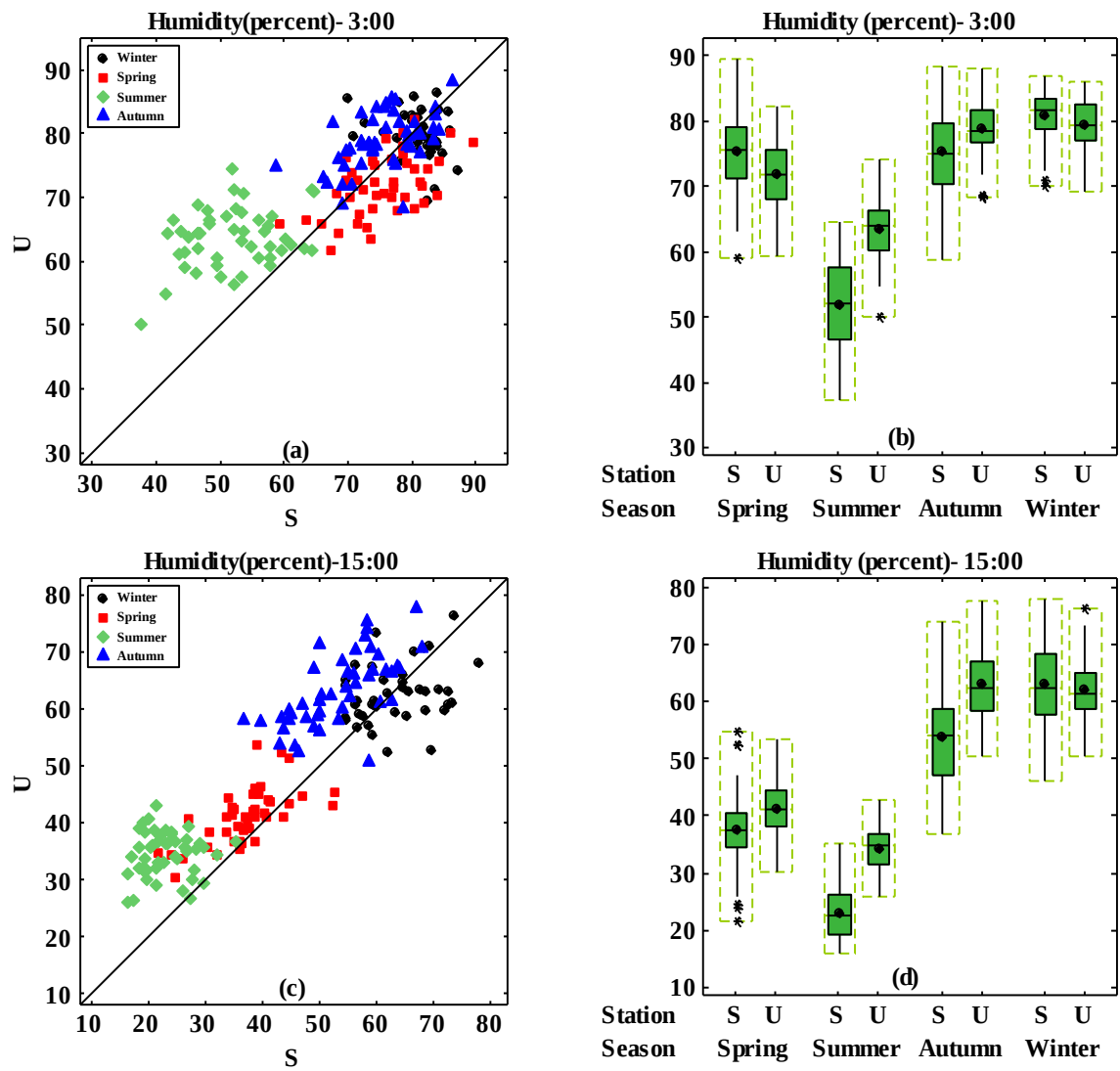
Figure S1. Seasonal patterns in relative humidity. Scatter plots of relative humidity at a) 03:00 h and c) 15.00 h in the different seasons at Urmia station (U) and Sazez station (S). b, d) The corresponding boxplots.
