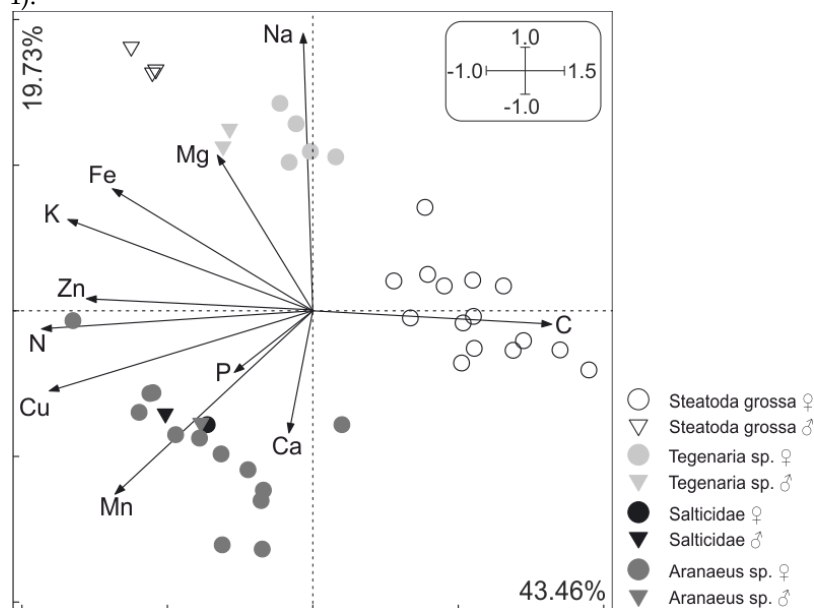
Figure 1. PCA plot—Multivariate analysis of stoichiometric relations in spider taxa and sexes. The first two axes are presented. Considering the 1 st axis, females are separated from males primarily due to their relatively high concentration of C and low concentrations of N, Cu, K and Zn (see Table 1 and Figure 2 for detailed statistics). Similarly, Steatoda grossa is separated from the other taxa due to its relatively high concentration of C and low concentrations of N, Cu, K and Zn (the other taxa do not differ statistically from each other; see Table 1 and Figure 3 for statistics). Considering the 2 nd axis, Tegenaria sp. forms a separate cluster mainly due to its relatively high concentrations of Na and Mg and low concentration of Mn. Opposite tendency is observed for Araneus sp., while Steatoda grossa together with Salticidae forms one cluster with intermediate concentrations of Na, Mg and Mn. These tendencies were confirmed by ANOVA performed independently for the 1 st and 2 nd axis scores ( p < 0.05 ; Figures 2-4).
