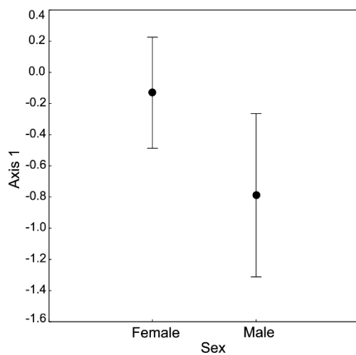
Figure 2. Multivariate analysis of stoichiometric relations in two sexes of spiders (PCA). ANOVA performed for the 1st axis scores ( F=4.46 , p=0.04 ). Bars denote confidence intervals.
