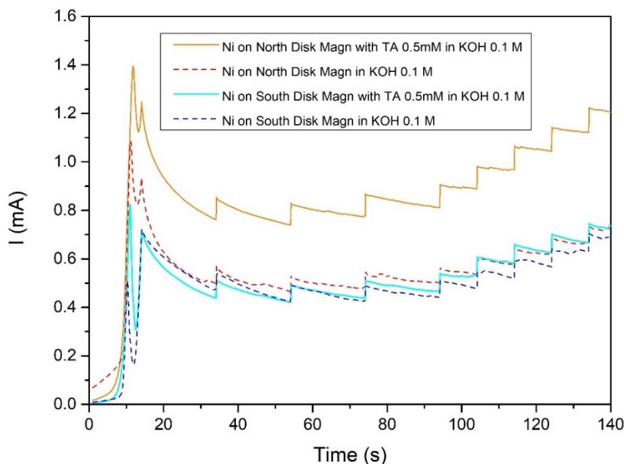
Figure 8 – Stepped sweeps curves recorded on a Ni deposited on magnet working electrode, a Pt sheet is the CE, Ag/AgCl/KCl is the RE. KOH 0.1 M aqueous solution the base electrolyte. First a potential ramp from 0 to 0.70 V at a 50 mV/s was applied, followed by eight +0.01 V potential steps, up to 0.78 V. The potential was maintained constant for 15 s between each step. L-(+)-tartaric acid concentration: ( blue dash ) South mag orientation 0 mM, ( red dash ) South mag orientation 0 mM, ( light blue ) South mag orientation 0.5 mM, ( orange ) North mag orientation 0.5mM
