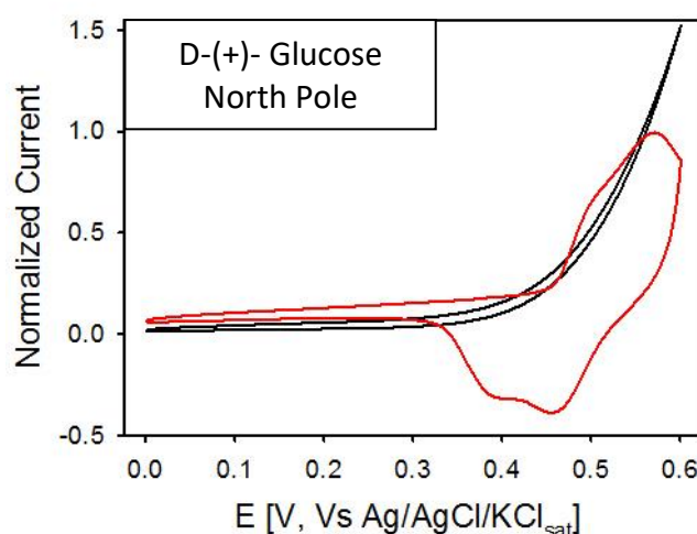
Figure 4 – Normalized cyclic voltammetry curves recorded with electrodeposited Ni on the North pole of the magnet. Red curve: KOH 0.1 M aqueous solution. Black curve: 0.1
