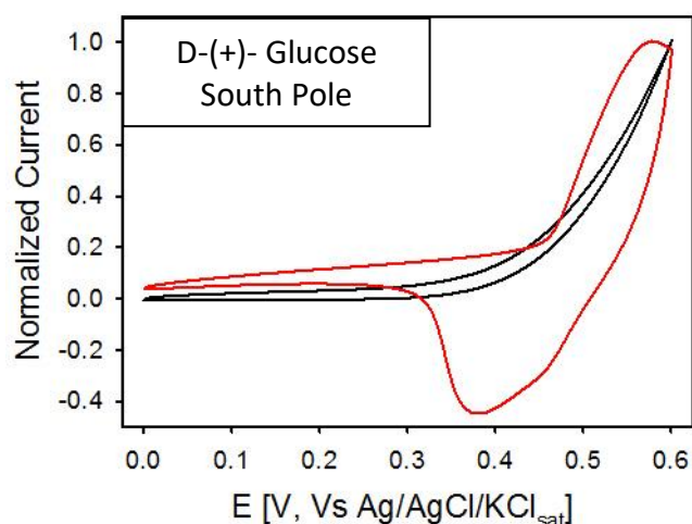
Figure 5 – Normalized cyclic voltammetry curves recorded with electrodeposited Ni on the south pole of the magnet. Red curve: KOH 0.1 M aqueous solution. Black curve: 0.1 M of D-(+)-Glucose in KOH 0.1 M aqueous solution. 50 mV/s potential scan rate, Pt as CE, Ag/AgCl/KCl as RE.
