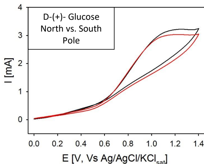
Figure 6 – Comparison between cyclic voltammetry curves recorded with electrodeposited Ni on both poles of the magnet. Red curve: south pole with 0.1 M of D-(+)-Glucose in KOH 0.1 M aqueous solution. Black curve: north pole with 0.1 M of D-(+)-Glucose in KOH 0.1 M aqueous solution. 50 mV/s potential scan rate, Pt as CE, Ag/AgCl/KCl as RE.
