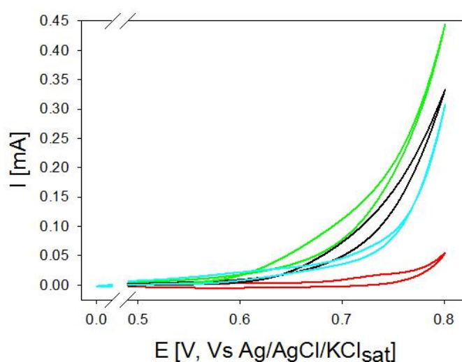
Figure 3 – Cyclic voltammetry curves recorded on a steel AISI 316L WE. 50 mV/s potential scan rate, Pt sheet as CE and Ag/AgCl/KCl sat as RE. KOH 0.1 M aqueous solution is the base electrolyte. D-(+)-glucose concentration: ( red ) 0 mM, ( light blue ) 1 mM, ( green ) 10 mM, ( black ) 100 mM.
