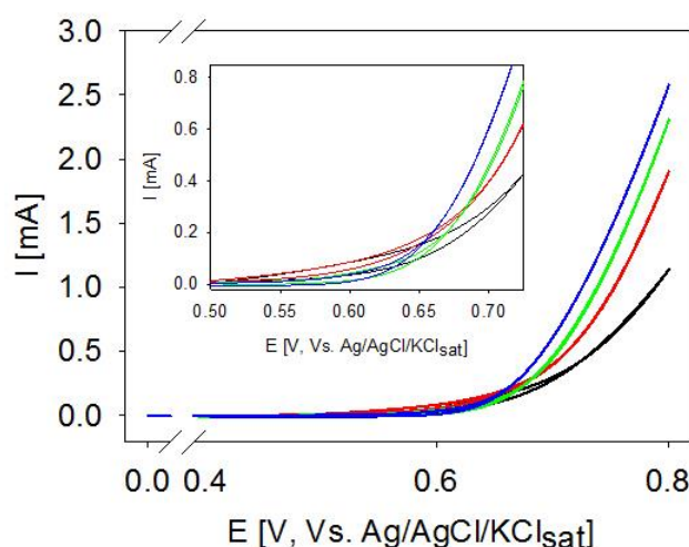
Figure 1 – Cyclic voltammetry curves recorded on a steel AISI 316L WE. 50 mV/s potential scan rate, Pt sheet as CE and Ag/AgCl/KCl sat as RE. KOH 0.1 M aqueous solution is the base electrolyte. L-(+)-tartaric acid concentration: (blue) 0 mM, (green) 0.5 mM, (red) 5 mM, (black) 25 mM. The inset shows the CV detail in the 0.5 and 0.75 V potential range.
