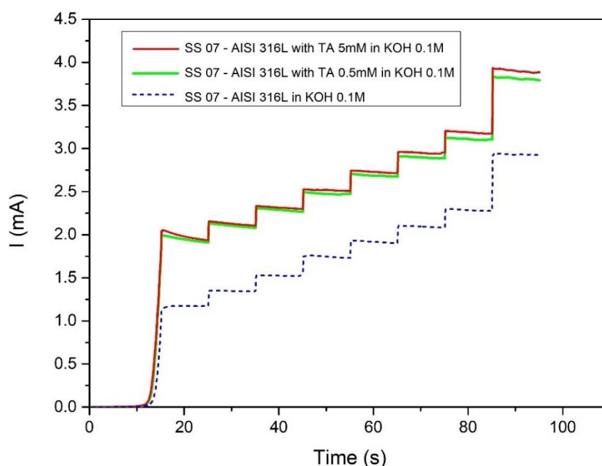
Figure 7 – Stepped sweeps curves recorded on a steel AISI 316L WE, Pt sheet as CE and Ag/AgCl/KCl sat as RE. KOH 0.1 M aqueous solution is the base electrolyte. A potential ramp from 0 to 0.75 V at a 50 mV/s was applied, followed by eight +0.01 V potential steps, up to 0.83 V. The potential was maintained constant for 10 s between each step. L-(+)-tartaric acid concentration: (blue dash) 0 mM, (green) 0.5 mM, (red) 5 mM
