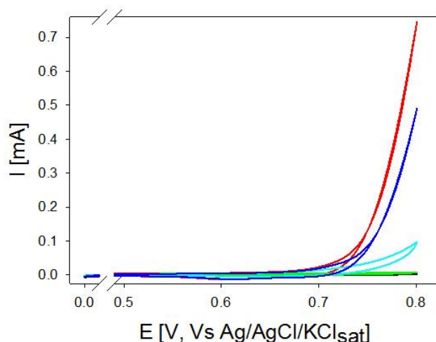
Figure 2 – Cyclic voltammetry curves recorded on a steel AISI 316L WE. 50 mV/s potential scan rate, Pt sheet as CE and Ag/AgCl/KCl sat as RE. KOH 0.1 M aqueous solution is the base electrolyte. L-(-)-aspartic acid concentration: ( red ) 0 mM, ( blue ) 1 mM, ( light blue ) 10 mM, ( green ) 50 mM, ( black ) 100 mM.
