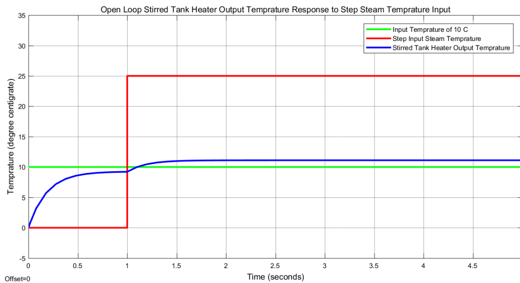
Figure 4 Open loop response
