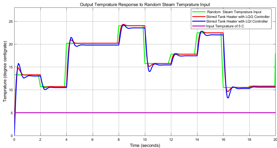
Figure 6 Closed loop response of the stirred tank heater with LQG and LQI controllers for a random steam temperature
