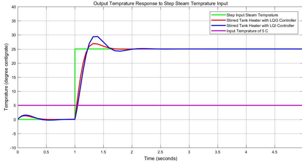
Figure 5 Closed loop response of the stirred tank heater with LQG and LQI controllers for a step steam temperature
