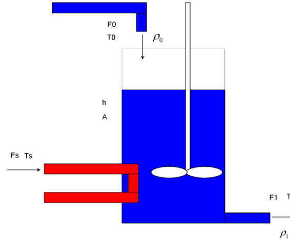
Figure 1 Stirred tank heater
