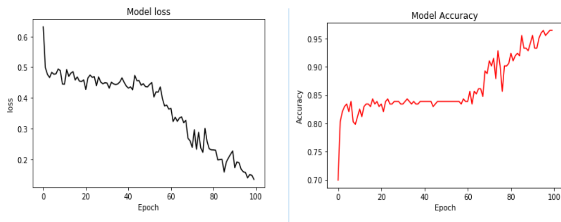
Fig.2. Accuracy and Loss plot obtained for each epoch
