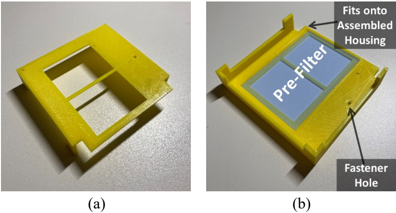
Figure 4. Pre-filter cover.
