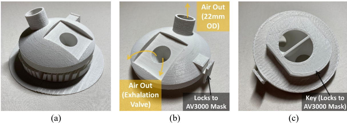
Figure 5. Respirator (a) Before cleanup; (b, c) After cleanup with design details
