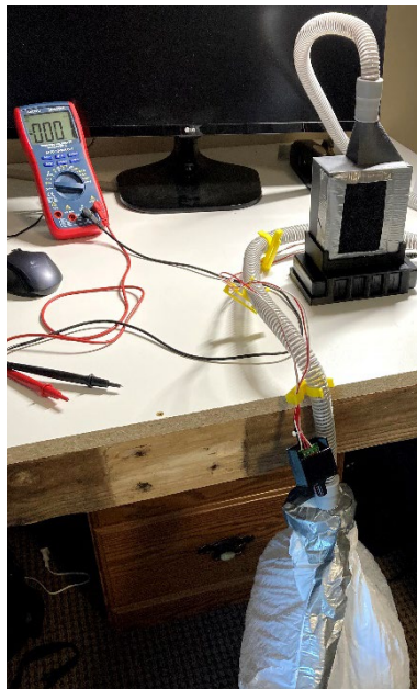
Figure 34. The airflow test setup, mid-test.
