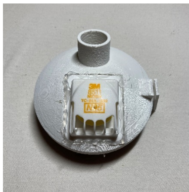
Figure 16. Glued 3M Cool-Flow exhalation valve in place.
