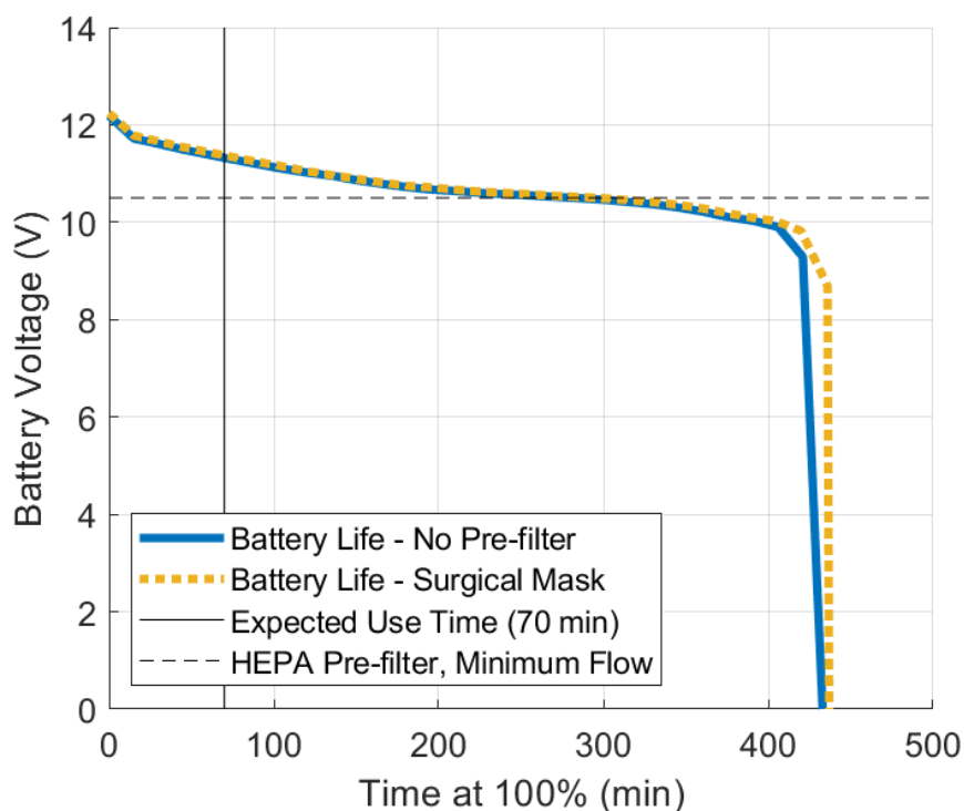
Figure 36. Battery voltage as a function of run time with no pre-filter and with a surgical mask prefilter.
