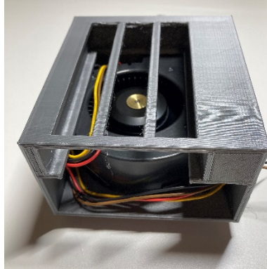
Figure 20. Properly run wire management.
