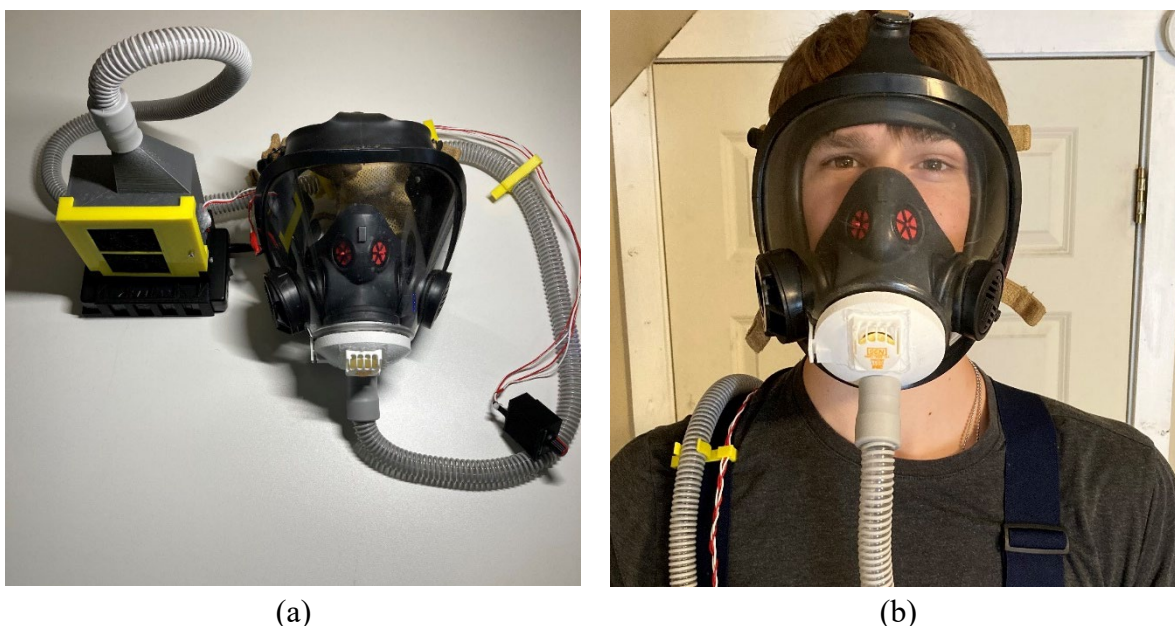
Figure 1. Fully assembled open source PAPR a) all components and b) in use.
