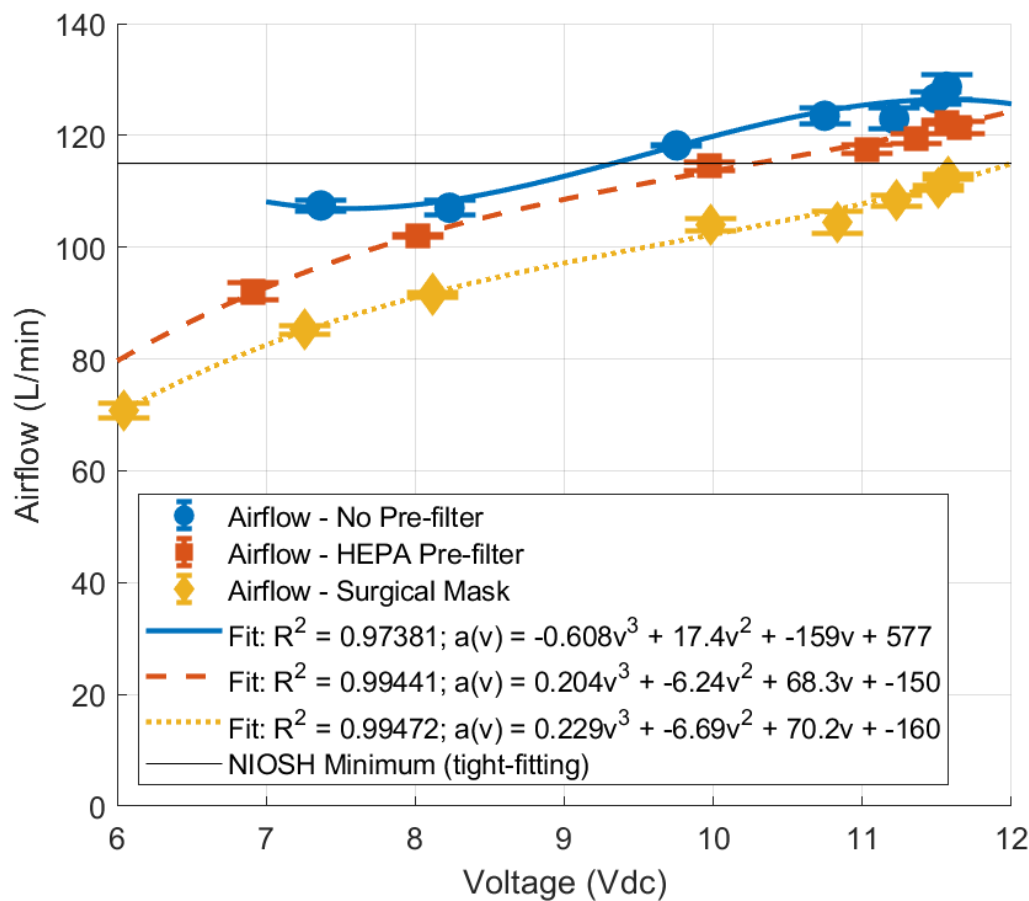
Figure 35. PAPR airflow test results
