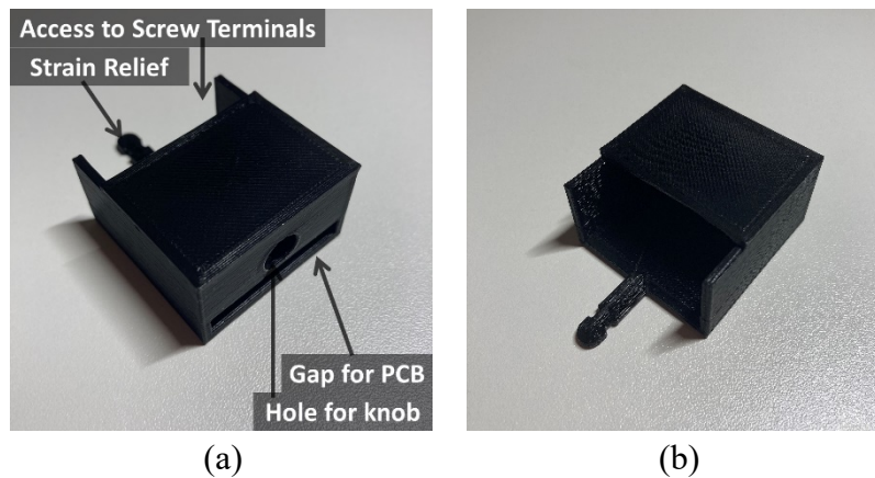
Figure 6. Controller Case (a,b) with design details.
