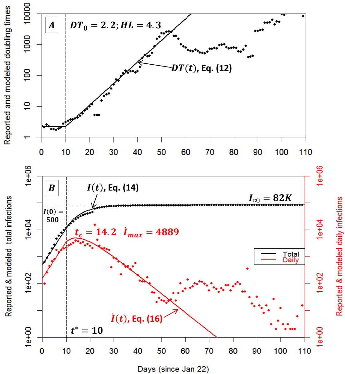
Figure 2: Panel A: Reported and modeled doubling times DT(t) in mainland China, from January 22 to May 11, 2020 (110 days). Panel B: Total reported and modeled numbers I(t) in black; daily reported and modeled numbers \dot{I}(t) in red (semi-logarithmic scales).
