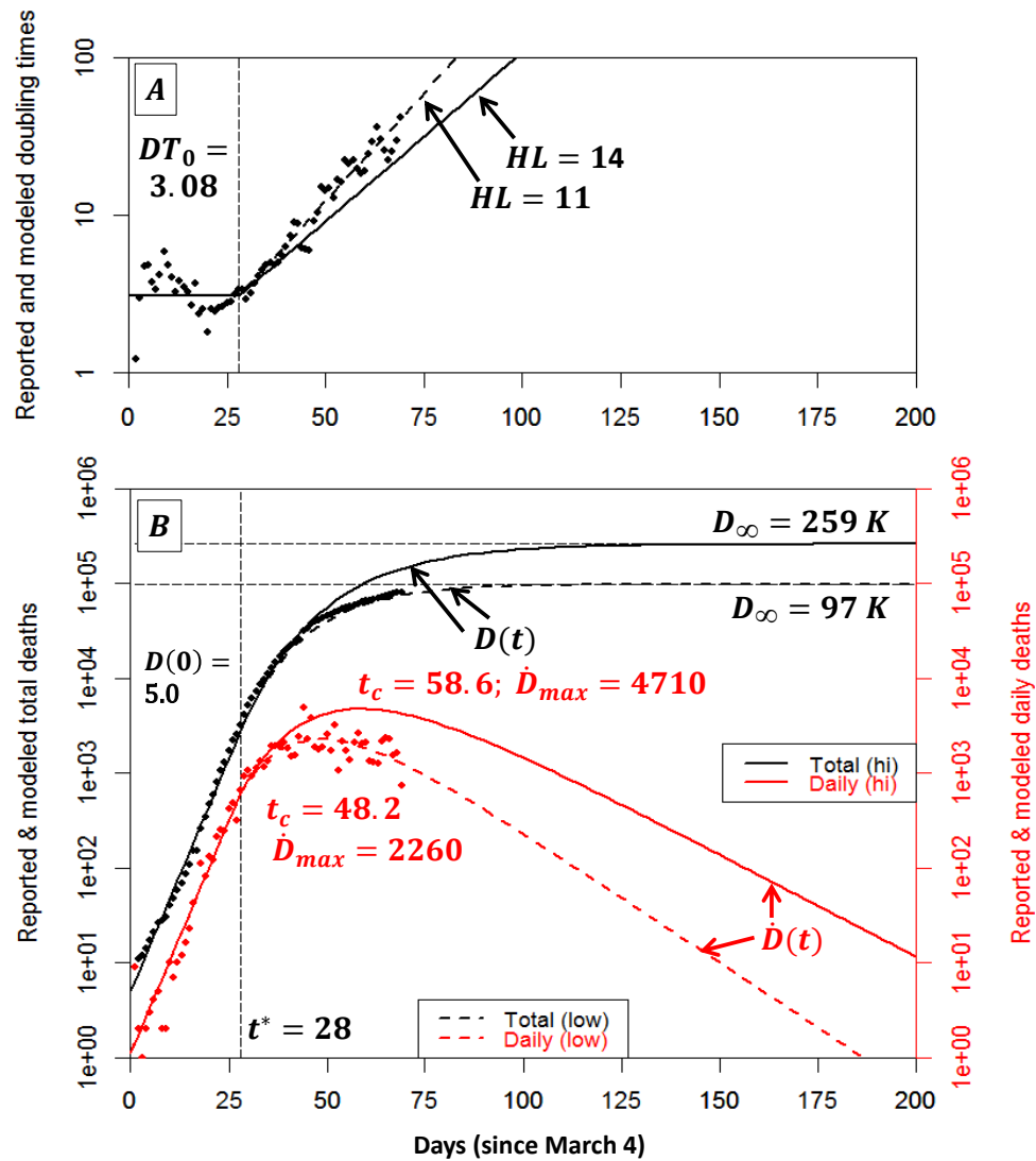
Figure 3: Panel A: Reported and low/high projected doubling times DT(t) for U.S. deaths from March 4 to May 11, 2020 (68 days). Panel B: Total reported and low/high projected total deaths D(t) in black; daily reported and low/high projected daily deaths \dot{D}(t) in red (semi-logarithmic scales).
