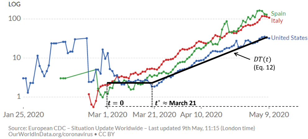
Figure 1: Doubling time of total confirmed Covid-19 cases for three countries - up to May 9, 2020 (logarithmic scale). The superimposed modeled DT(t) (black line) captures for the U.S. the pattern of a constant value DT_0 roughly from March 1 ( t = 0 ) to March 21 ( t^* = 21 ). For t > t^* the logarithm of DT(t) increases roughly linearly with slope \ln(2)/HL . (In Spain and Italy, where there appears to be little or no initial exponential stage, we might take a duration t^* = 0 for that stage).
