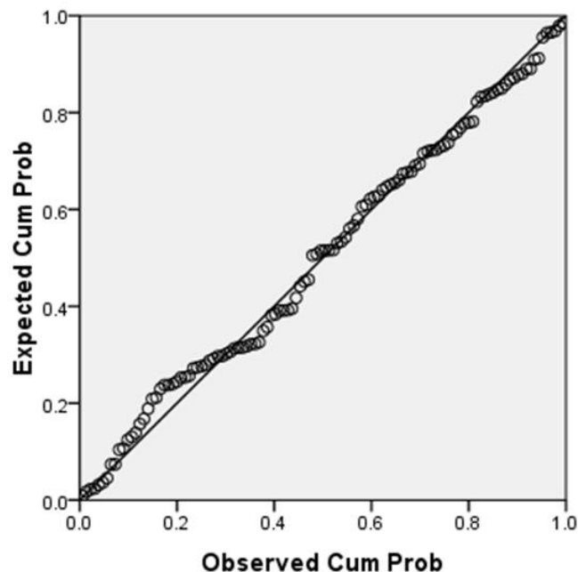
Figure 2. Normality probability plot: X-axis represents the observed and Y-axis represents the expected prob.
