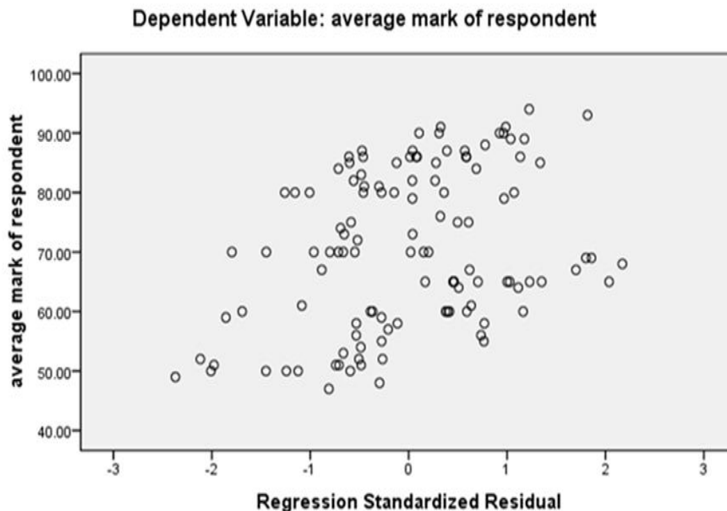
Figure 3. Scatter plot: X-axis represents the regression standardized residual and Y-axis represents the average mark of respondent.
