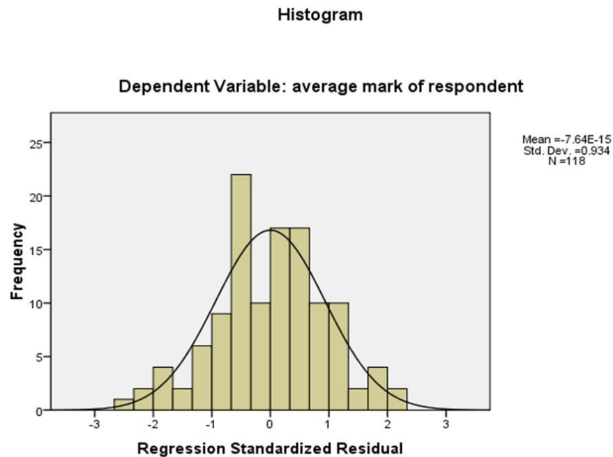
Figure 1. Histogram plot in bar chart depicting the normality assumption
