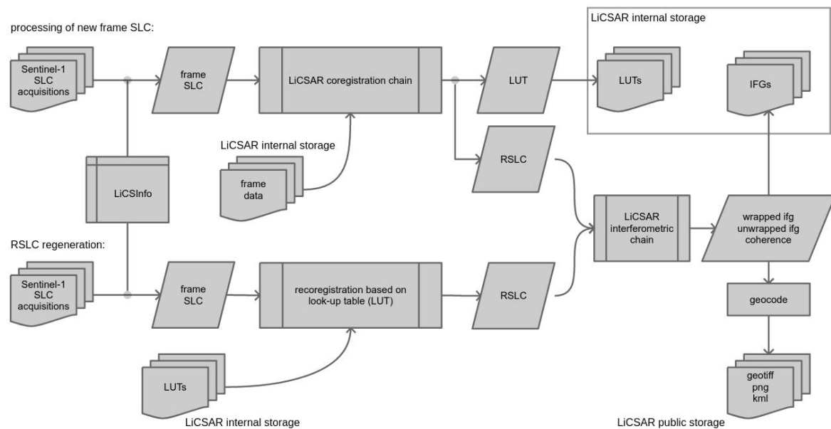
Figure 2. General flowchart of the LiCSAR processing chain
