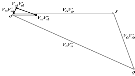
FIG. 1. A Figure representing the knowledge of our confined to the triangle, compared out the fourth-generation model in the context of CPV.
