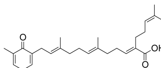
Sargaquinoic acid
