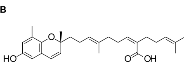
14,15,18,20-diepoxyturbinarin
