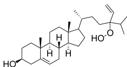
24-hydroperoxy-24-vinyl-cholesterol
