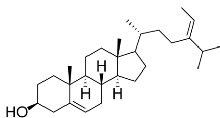
Fucosterol
