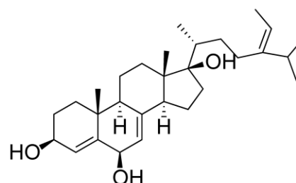
3,6,17-trihydroxy-stigmasta-4,7,24(28)-triene
