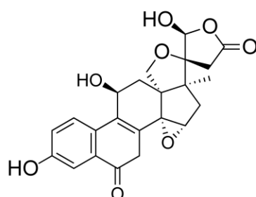
14,15,18,20-diepoxyturbinarin
