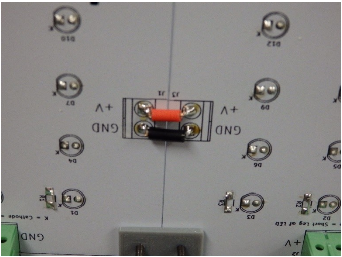
Figure 8. Wires directly soldered to transfer power from one board to the next
