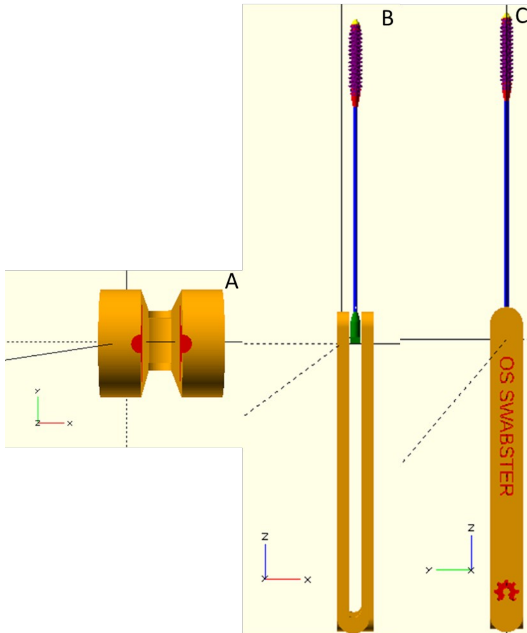
Figure 4. OpenSCAD rendering of A) lengthwise view of clamping section of tong handle; B) tong handle showing swab placement in relaxed state for easy removal; and C) swab and handle assembled in side profile with customizable writing.
