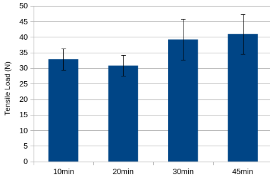
Figure 26. Maximum tensile load at break for open source swabs as a function of UV curing time.
