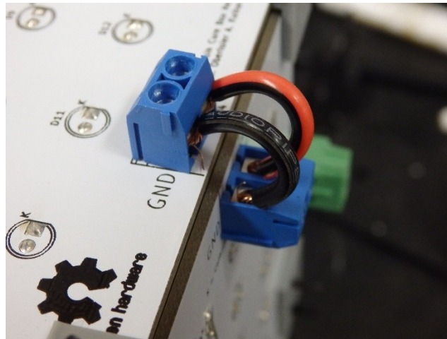
Figure 10. Wires connecting two terminal blocks on a corner. The wires are made longer than necessary as they double as the hinge for the lid.
