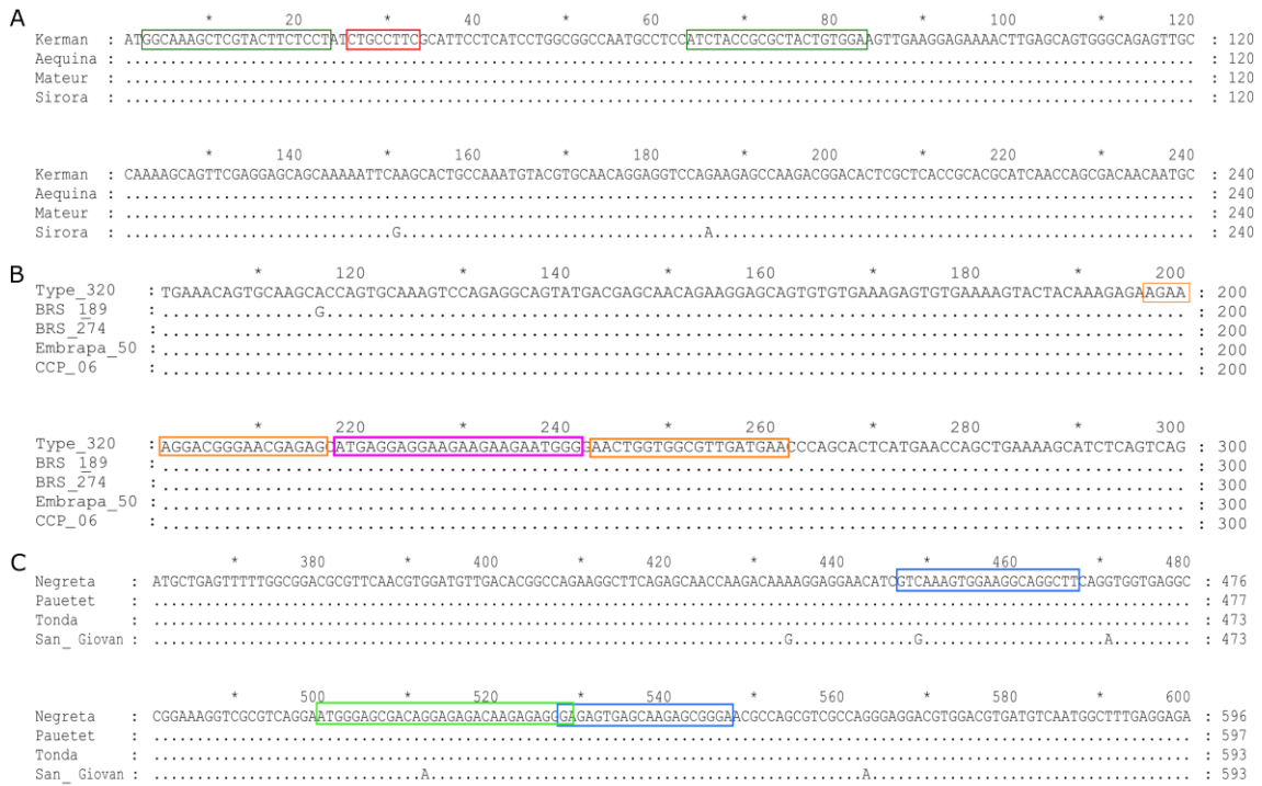
Figure S1. Partial alignment of Pis v 1, Ana o 1 and Cor a 9 coding sequences. Alignment (performed with Clustal Omega) of pistachio (A), cashew (B) and hazelnut (C) varieties of real time PCR targets. Position and sequence of primers and probes are squared. Nucleotide identities are dots in the alignment.
