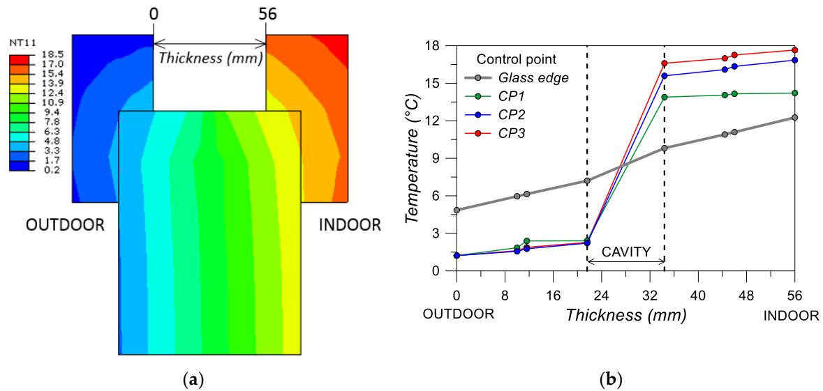
Figure 14. Numerical thermal performance assessment of a full-size CLT–glass façade element. Temperature distribution: (a) in the frame cross-section (legend values in °C) and (b) in glass thickness (with CP n = 1, 2, and 3 diagonal control points at a distance of 50 mm, 90 mm, and 150 mm from the corner; ABAQUS).
