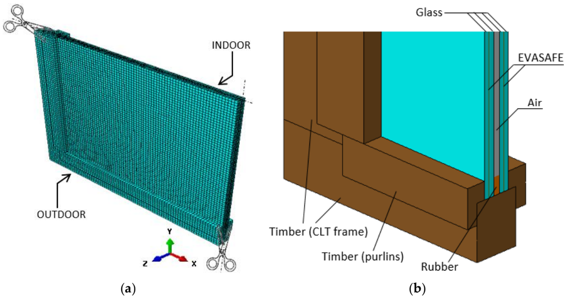
Figure 12. Reference FE model for the thermal assessment of full-size CLT–glass façade elements: (a) global assembly (1/4th the nominal geometry) and (b) a detailed view with a hidden mesh (ABAQUS).
