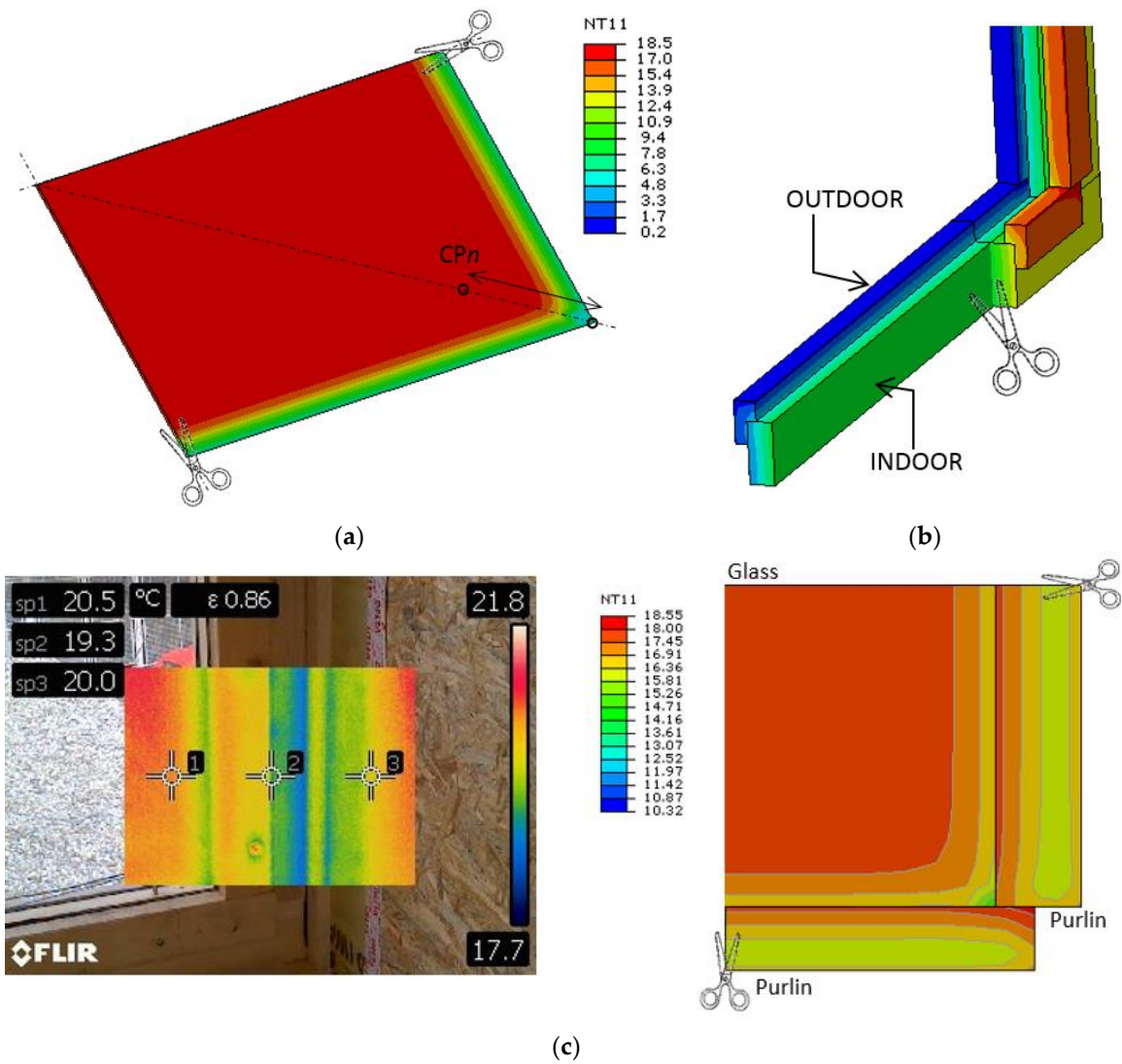
Figure 13. Numerical thermal performance assessment of a full-size CLT-glass façade element (ABAQUS). Expected distribution of temperature (a) in the internal glass panel (external side with
