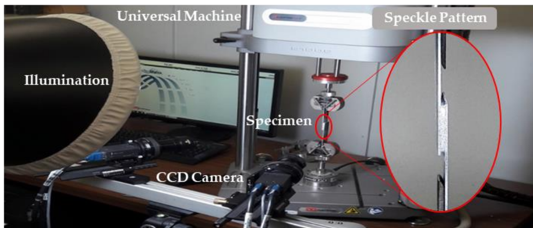
Figure 3. Experimental set-up of 3D Digital Image Correlation
