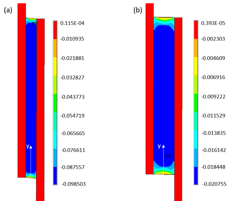
Figure 10. Shear strain field obtained by numerical simulation using the Mooney Rivlin constitutive model.(a) 2mm and (b) 4mm of PDMS thickness.
