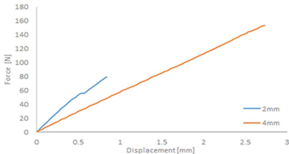
Figure 6. Force-displacement curve for the shear test
