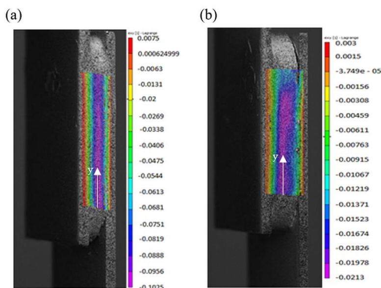
Figure 9. (a) Shear strain field for a 2mm thickness PDMS plate; (b) Shear strain field for a 4mm thickness PDMS plate
