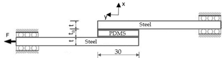
Figure 2. The specimen used in the simple shear test
