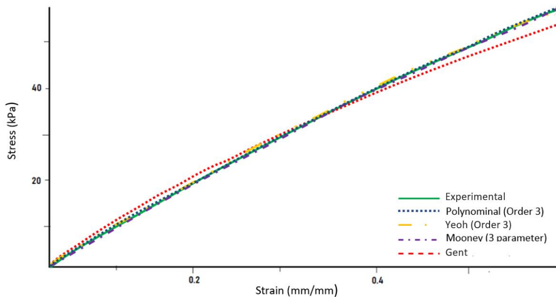
Figure 4. Stress-Strain curve solution for different constitutive hyperelastic mathematical models
