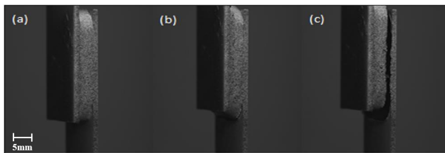
Figure 8. Image of 4mm PDMS thickness: a) before deformation; b) beginning of rupture; c) after rupture.
