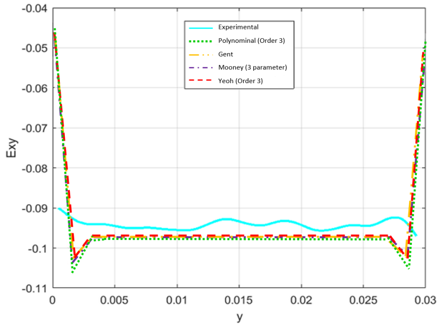
Figure 11. Shear strain obtained numerically and experimentally along the y-direction for 2 mm of PDMS.
