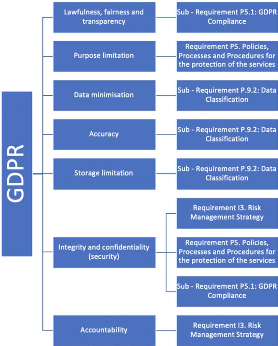
Figure 4. GDPR Mapping
