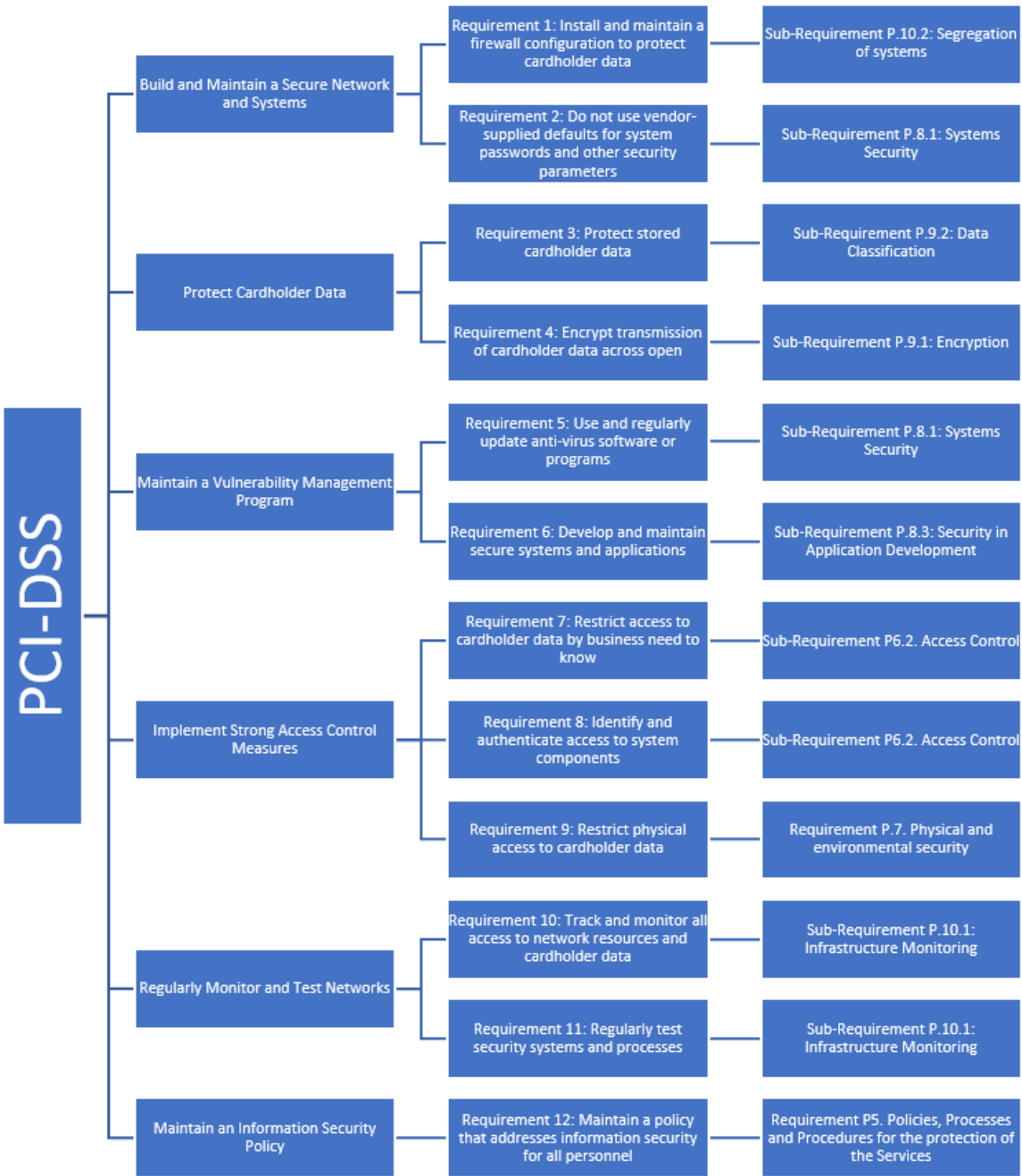
Figure 5. PCI-DSS Mapping
