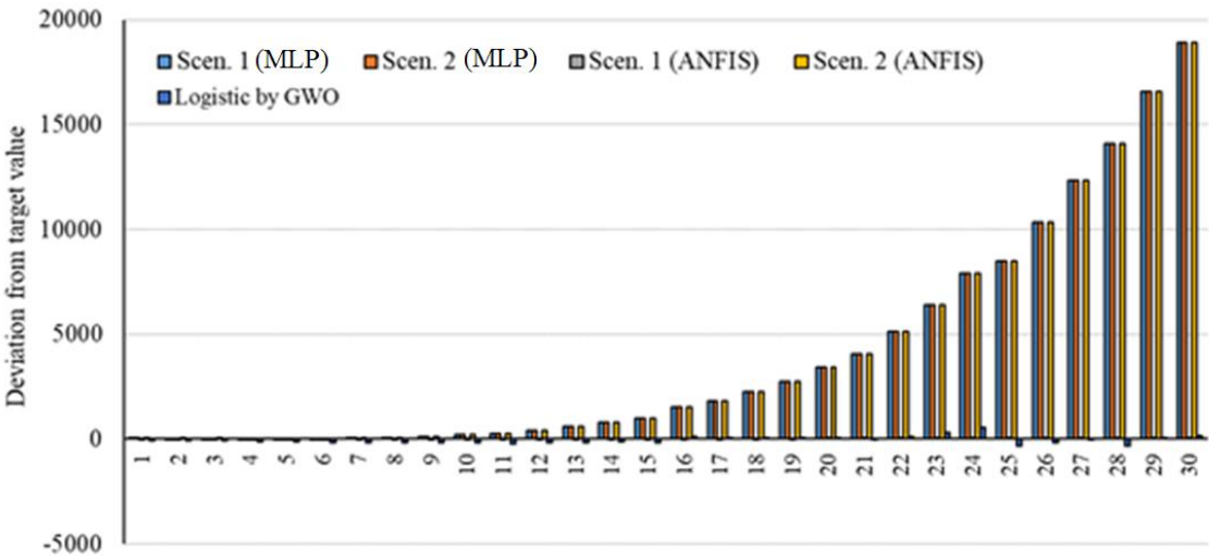
Figure 17. Deviation from target value for models related to Italy
