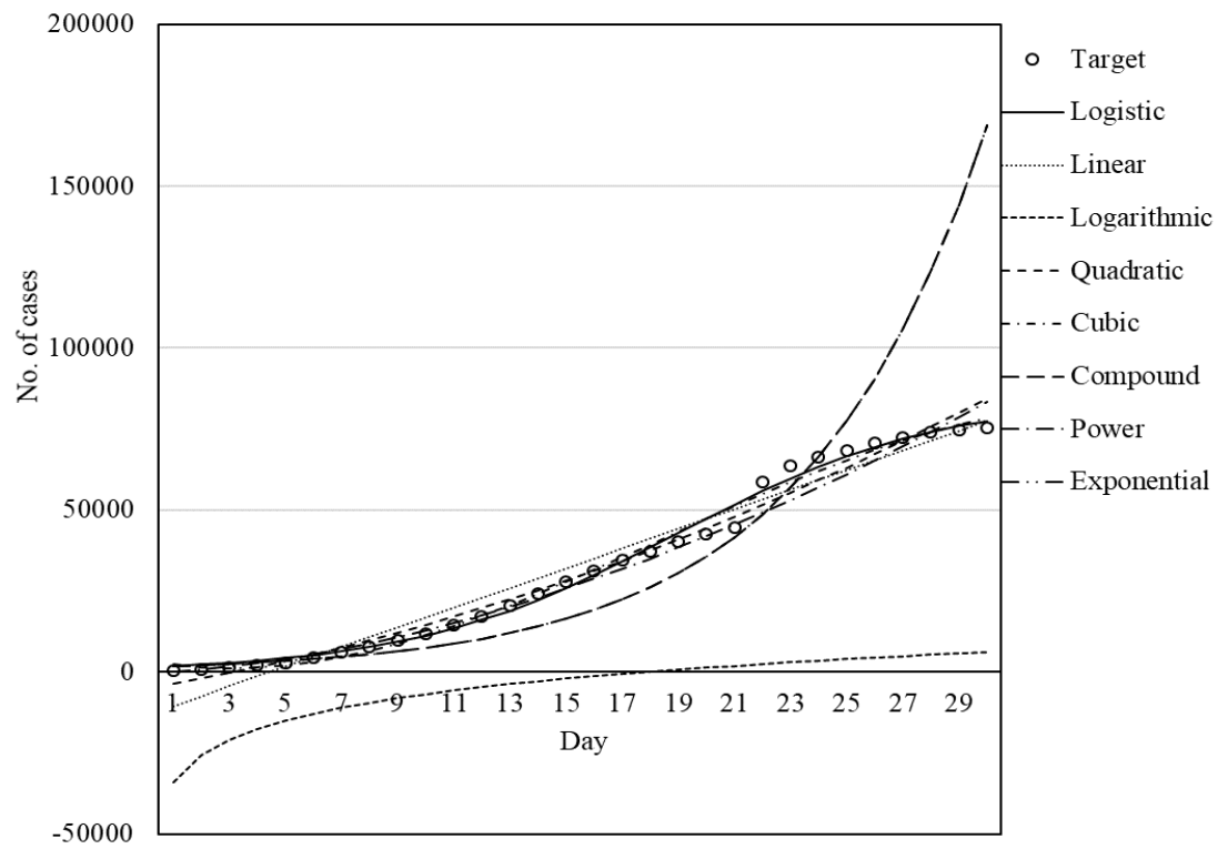
Figure 7. Fitness graph for China fitted by GWO
