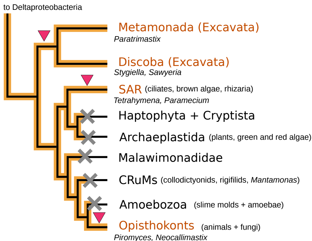
Figure 2: Schematic tree of presence and absence of SHC/STC in eukaryotes.
