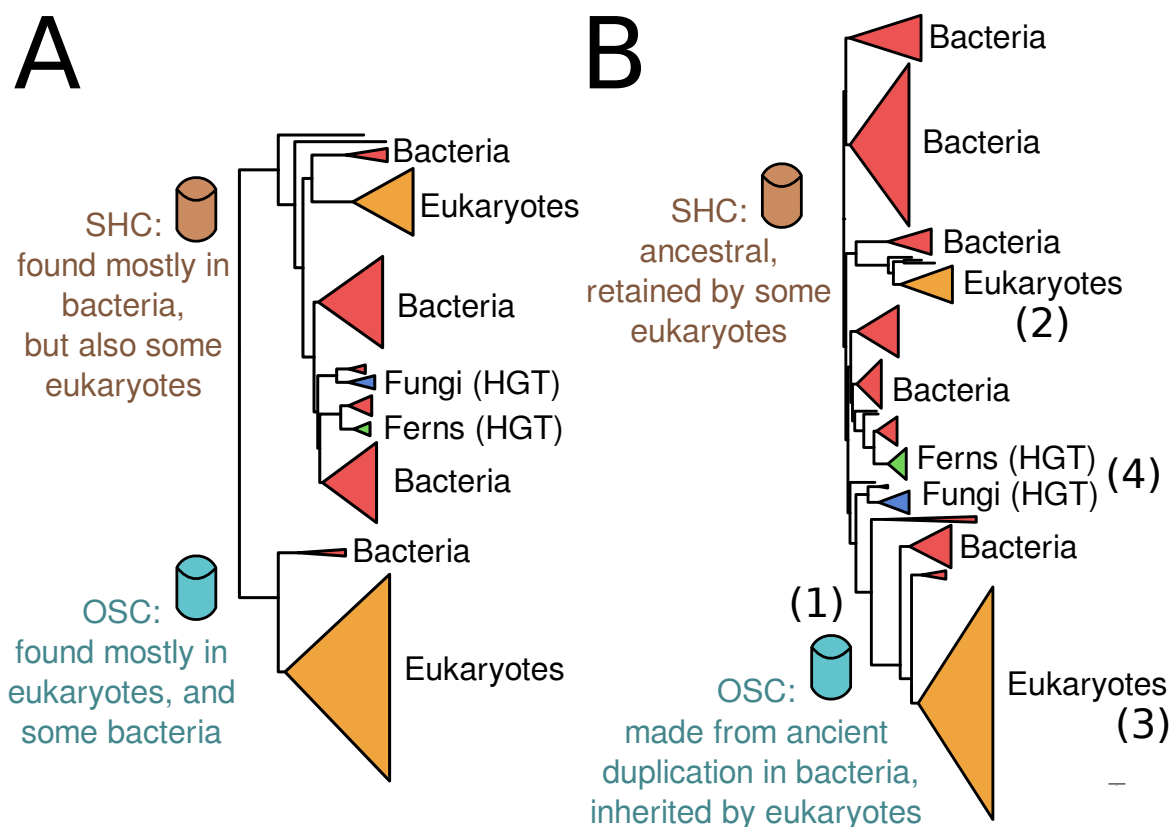
Figure 1: Schematic tree of SHC and OSC evolution.
