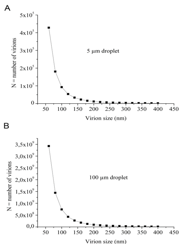
Figure 1: Number of virions N vs virion diameter d(\text{nm}) in droplets of 5 and 100 \mu\text{m} . For a 5 \mu\text{m} droplet, the virion number will be in the order of 10^5 from 60-100 nm; for a 100 \mu\text{m} particle the number will be about 10^9 . Thus, the difference in particle number is around 4 orders of magnitude between a particle of 5 \mu\text{m} (aerosol) and a particle of 100 \mu\text{m} (droplet). This may explain why an airborne infection is less likely to occur. However, crowded areas and with poor ventilation could make the difference, since virions could reach enough concentration and the probability of infection will increase with time and with the time of exposure. For this reason, health personnel are with the higher risk. A: number of virions in a 5 \mu\text{m} droplet. B: number of virions in a 100 \mu\text{m} droplet. Thus, the efficient packaging makes the difference.
