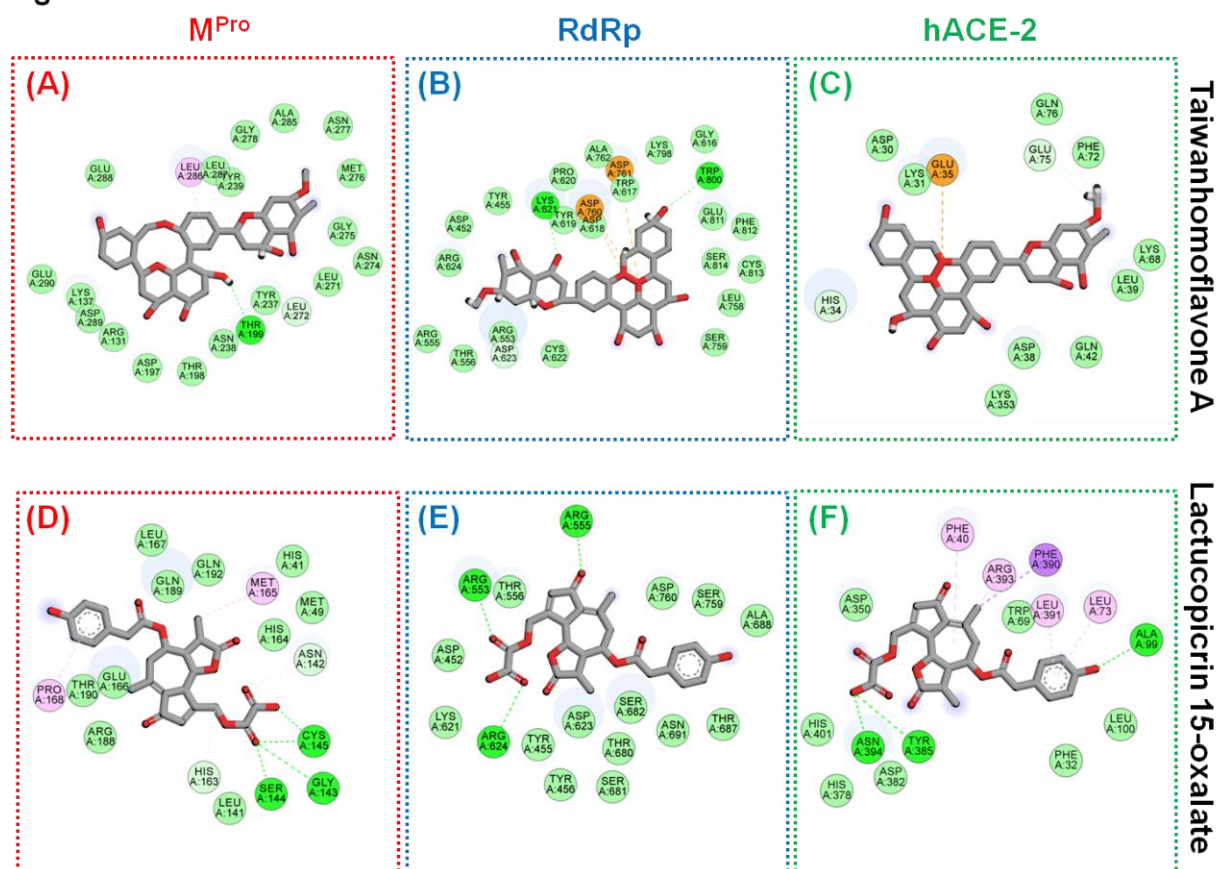
Figure 7. Intermolecular interaction between Taiwanhomoflavone A with active site residues of (A) MPro, (B) RdRp and (C) hACE-2. Next is the interaction map of Lactucopicrin 15-oxalate with (D) MPro, (E) RdRp and (F) hACE-2. The representation of the interaction between different residues is similar to Figure 6.
