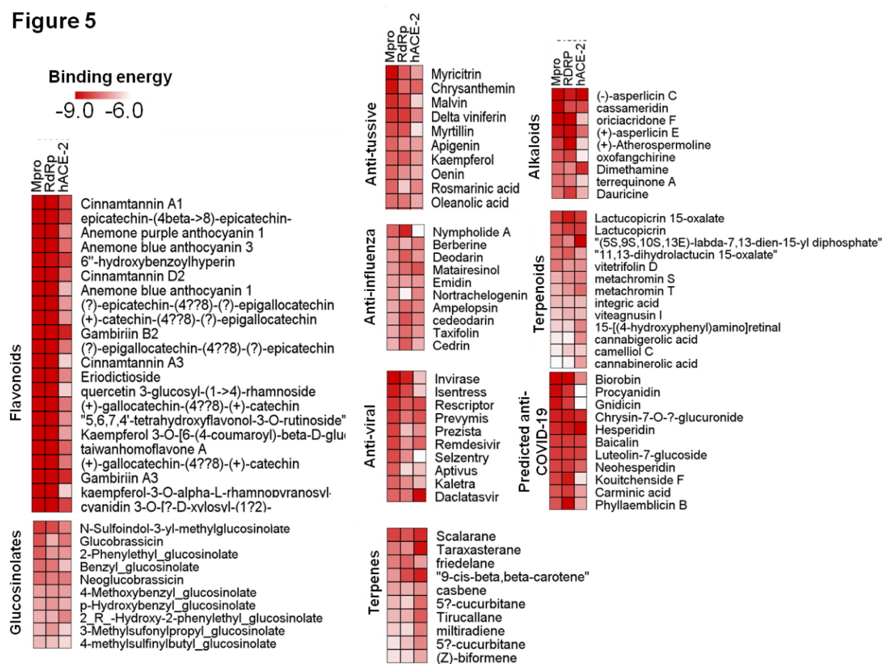
Figure 5. Heatmap of binding energies of top hits for different types of molecules used for screening, namely flavonoids, glucosinolates, anti-tussive, anti-influenza, synthetic anti-viral, terpenes, terpenoids and alkaloids. In general, we noticed strong binding of ligands towards M Pro and RdRp as compared to the hACE 2 receptor. Flavonoids showed promising results with better binding affinities than existing synthetic anti-viral drugs.
