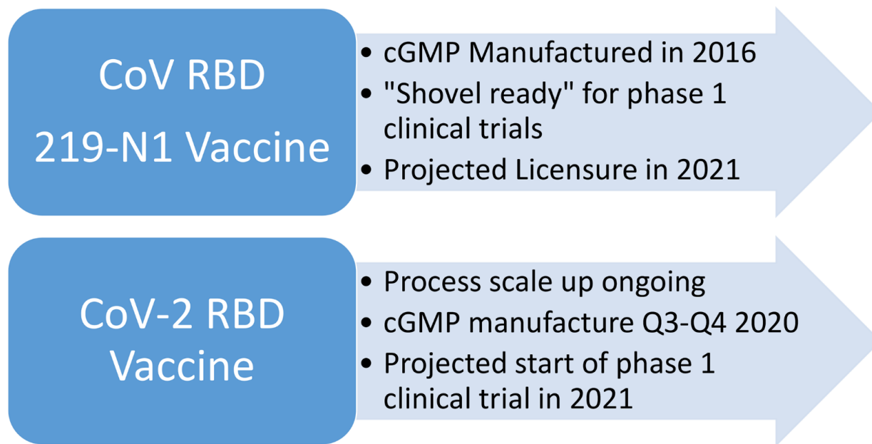
Fig 1. Estimated timelines of Coronavirus RBDs as COVID-19 vaccines (Fig 1)
