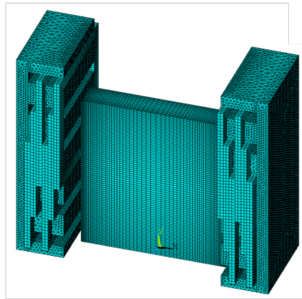
Figure 2. Numerical model geometry and finite element mesh for electromagnetic computation.
