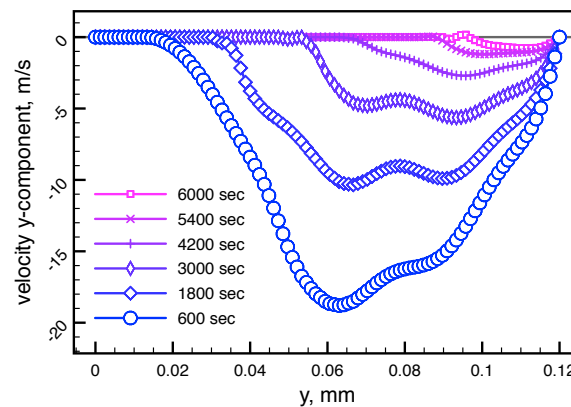
Figure 8. Melt velocity decreasing during solidification.
