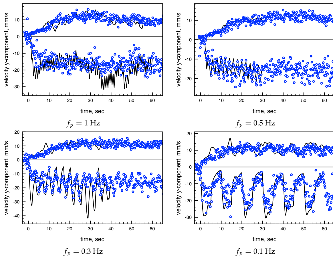
Figure 10. Spin-up liquid metal velocities at different pulsation frequencies. Dots – measured; lines – calculated. Video files of simulations can be found at supplementary data http://dx.doi.org/10.17632/7fmy5kh278.1
