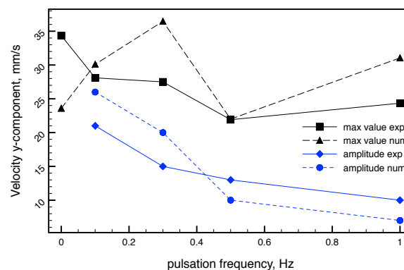
Figure 12. Dependences of liquid metal flow parameters on TMF pulsation frequency.
