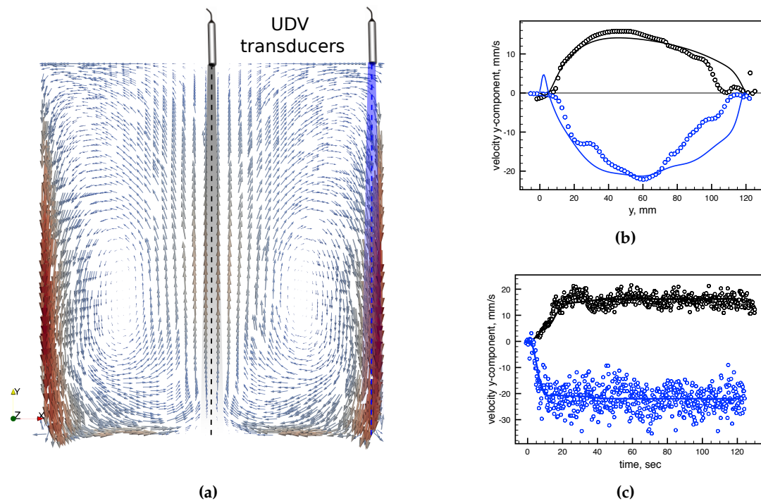
Figure 6. (a) – velocity field of liquid metal under TMF impact with UDV transducers placement. (b) – mean velocity profile (dots - experimental, line - numerical), (c) – velocity dynamics (blue - near the wall, black - central axis)
