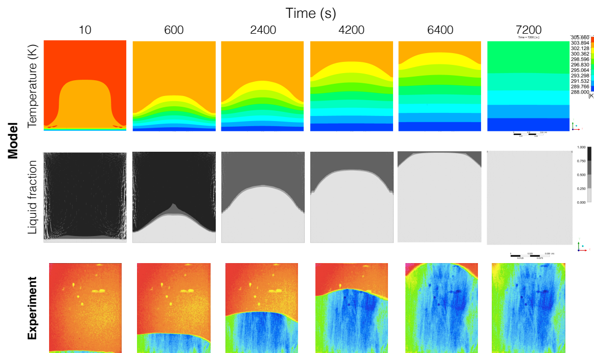
Figure 7. The solidification process dynamics in the presence of a travelling magnetic field. The animation of transient solidification can be found at supplementary data http://dx.doi.org/10.17632/7fmy5kh278.1 .
