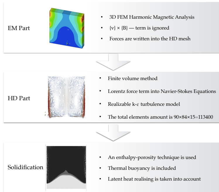
Figure 3. Numerical scheme for the solidification process in presence of TMF.
