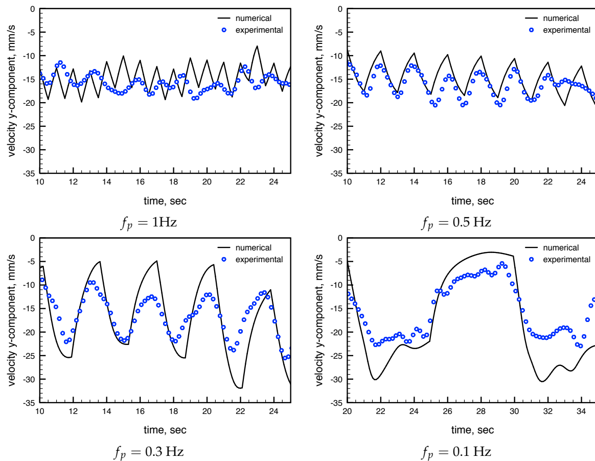
Figure 11. Comparison of experimentally and numerically obtained velocities (after FFT smooth) at different pulsation frequencies. Animations of transient calculations can be found at supplementary data http://dx.doi.org/10.17632/7fmy5kh278.1
