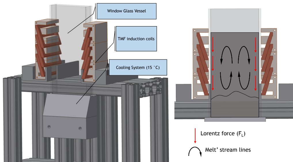
Figure 1. Experimental setup of solidification process in presence of travelling magnetic field from [10].
