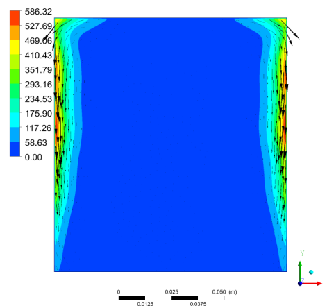
Figure 5. Cut surface of liquid metal volume with Lorentz forces [N/m 3 ].
