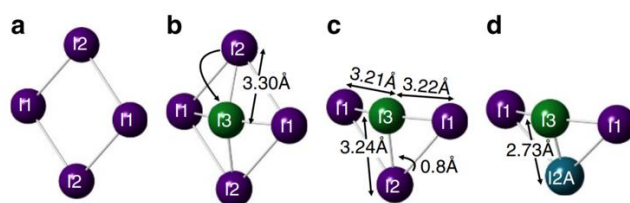
Figure 6. Proposed mechanism for I 2 formation in MAPbI 3 . (a) (110) plane of perovskite showing four I - ions. (b) Iodine at I 2 position moves to interstitial I 3 position. (c) I 3 is now surrounded by three iodine ions at approximately same distances. (d) This leads I 2 to move to the I 2A position, creating a bond and producing a I 2 molecule (bond between I 3 and I 2A ). Reproduced with permission from Nat. Commun. 2017 , 8, 15152. Reference [14].
