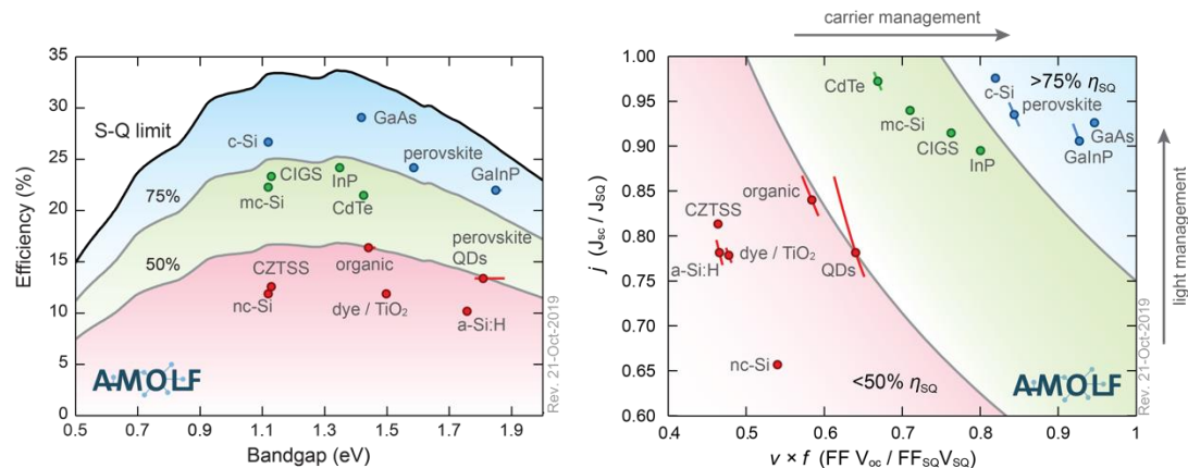
Figure 4. Record-efficiency cell parameters compared to the detailed-balance limit. (a) Blue dots show materials that are closer to the Shockley-Queisser (SQ) detailed-balance limit (black line). Green and red dots (area) show the materials that are performing less good. (b) SQ-Normalized current vs normalized voltage ( \times fill factor) indicates in which aspects materials could be improved: CdTe is close to the current limit, but loses out on voltage (which can be optimized by charge carrier management). GaInP gives an excellent voltage, but needs better light management (converting photons into electrons/current) to be improved. Reproduced with permission from Science 2016 , 352, aad4424. Updated graphs, taken from the website related to Reference [10].
