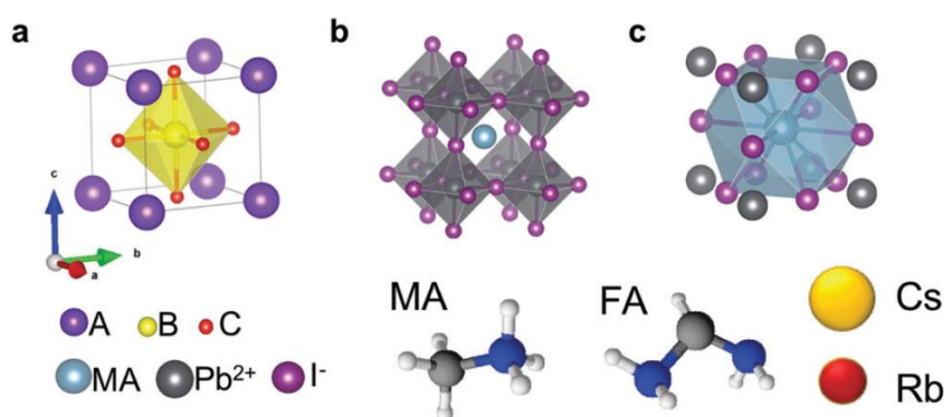
Figure 1. Representation of the typical components of lead perovskites and the typical perovskite crystal structure, viewed in three different ways. ABX_3 (or ABC_3 ) with A components being MA, FA or Cs(I) or Rb(I), the B = Pb(II). The X (or C) can be iodide (I - ), bromide or chloride. Note that the octahedral coordination around Pb(II) can be displayed centrally (a) or the MA can be shown centrally (b). In (c) the square unit cell is shown with MA in the center. Reproduced with permission from Energy Environ. Sci 2017, 10(3), 710-727, Reference [2].
