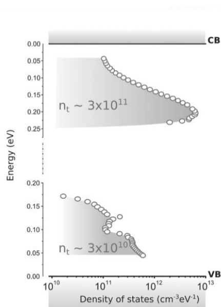
Figure 5. Density of the trap states (with their energetic distribution) within the band gap, extracted from the temperature-dependent properties. The valence band has less traps, with a slightly smaller energy distribution. Reproduced with permission from Adv. Mater. 2016 , 28, 3406–3410. Reference [12].
