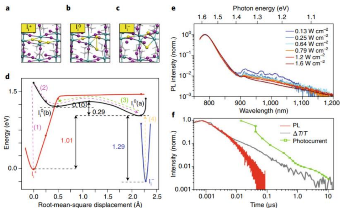
Figure 9. Interstitial iodine defects as hole and electron traps in MAPbI 3 . Local geometrical structures of interstitial iodine (a) as a cation I_i^+ , (b) as a neutral atom, I_i^0 , and (c) as iodide, I_i^- . (d) Potential energy landscapes related to species in (a), (b) and (c). Root mean square displacement of iodine atom with respect to the position of I_i^+ . Dots are calculated points, lines are interpolated. (e) Steady-state photoluminescence (PL) spectra with increasing excitation fluence, showing enhanced NIR (~1000 nm) emission at low excitation powers. (f) Photoluminescence dynamics probed at 1.56 eV, together with photocurrent decay and transient absorption kinetics. Reproduced with permission from Energy Environ. Sci. 2018 , 11 , 702–713. Reference [22] as well as Reproduced with permission from Energy Environ. Sci. 2016 , 9 , 3472–3481. Reference [8].
