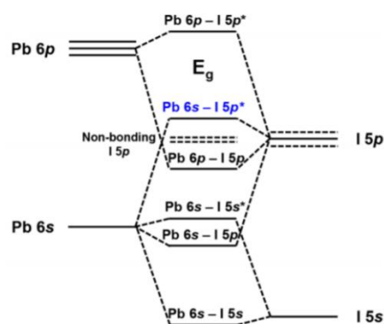
Figure 14. Band gap of \text{MAPbI}_3 . The orbital contributions of Pb and I. Reproduced with permission from Chem. Mater. 2016 , 28, 4259–4266. Reference [44].
