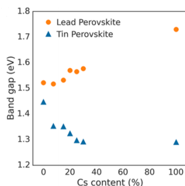
Figure 13 Optical band gap as function of cesium content for perovskites (\text{FA}_{1-x}\text{Cs}_x)\text{MI}_3 , with \text{M} = \text{Pb} or \text{M} = \text{Sn} . Reproduced with permission from J. Am. Chem. Soc. 2017 , 139, 11117–11124. Reference [42].
