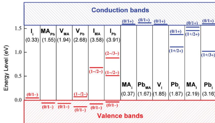
Figure 7. Calculated transition energy levels of various types of point defects in MAPbI 3 (interstitials (I), ion substitutions and vacancies (V) are indicated). The formation energies of neutral defects are shown in parentheses. The acceptors (red, trapping electrons) and donors (blue, trapping holes) are ordered by the formation energies (from left to right). Reproduced with permission from Adv. Mater. 2014 , 26, 4653–4658. Reference [17].
