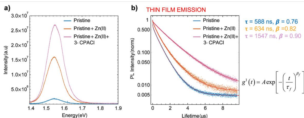
Figure 11. Characterization of MAFA film with and without Cl − and Zn(II) dopants. (a) Relative yield of emission by time-integrated PL spectra. (b) Time-dependent PL traces with different dopants, stretched exponential fitting with function. Reproduced with permission from ACS Appl. Mater. Interfaces 2019 , 11 , 17555–17562. Reference [41].
