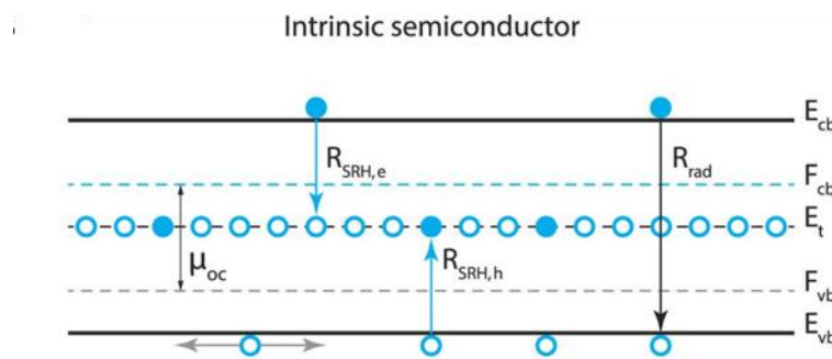
Figure 2. Electron and hole energetics and recombination. The free energy \mu_{oc} of photogenerated electron-hole pairs at open circuit (oc) is equal to the energy splitting of the quasi-Fermi level conduction ( F_{cb} ) and valence ( F_{vb} ) bands. The trap level ( E_t ) in the mid-gap is empty from where Shockley-Read-Hall recombination of electrons (holes), R_{SRH,e} ( R_{SRH,h} ), occurs. Reproduced with permission from Sci. Rep. 2017 , 7, 44629. Reference [6].
