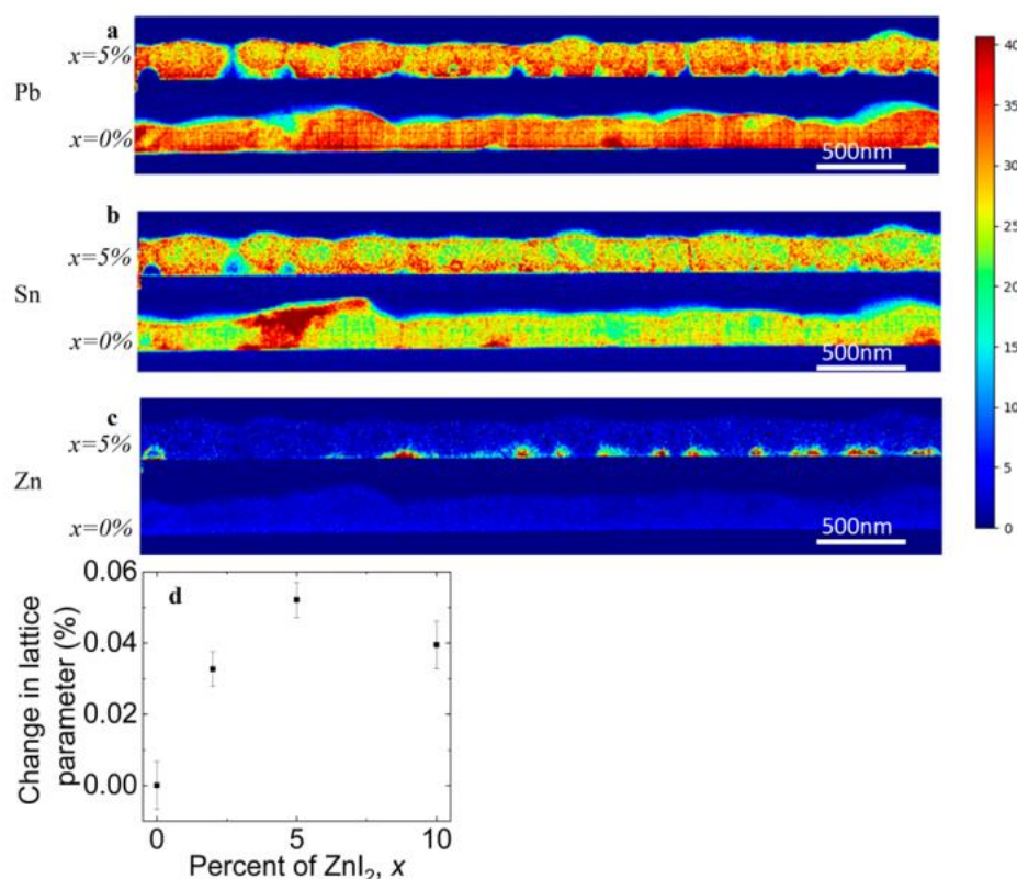
Figure 10. Distribution of elements of FA(Pb 0.5 Sn 0.5 )I 3 with and without 5 % ZnI 2 added measured by STEM/EDX. (a) Pb. (b) Sn. (c) Zn. (d) Change in lattice parameter with doping content. Reproduced with permission from ACS Energy Lett. 2019 , 4 , 2301–2307. Reference [32].
