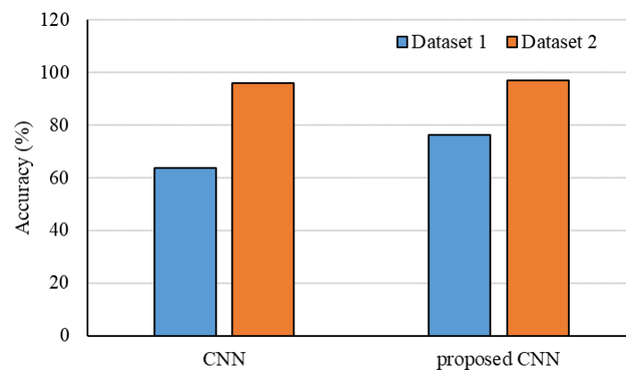
Fig. 18. Results for the study by De Sousa Ribeiro et al [106]
