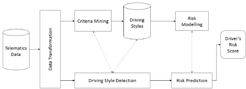
Fig. 15. The graph of the conceptual model [77]
