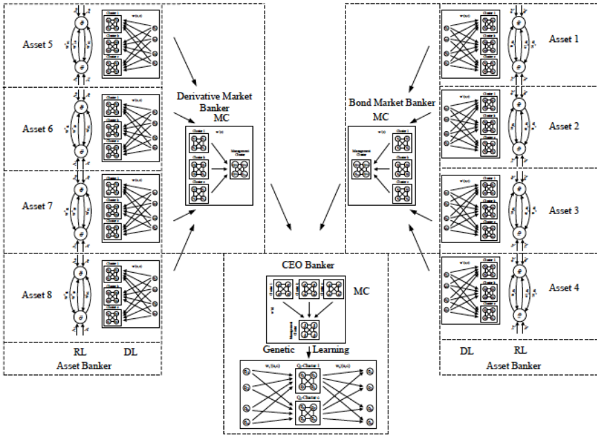
Fig. 18. Structure of smart investment model [102]
