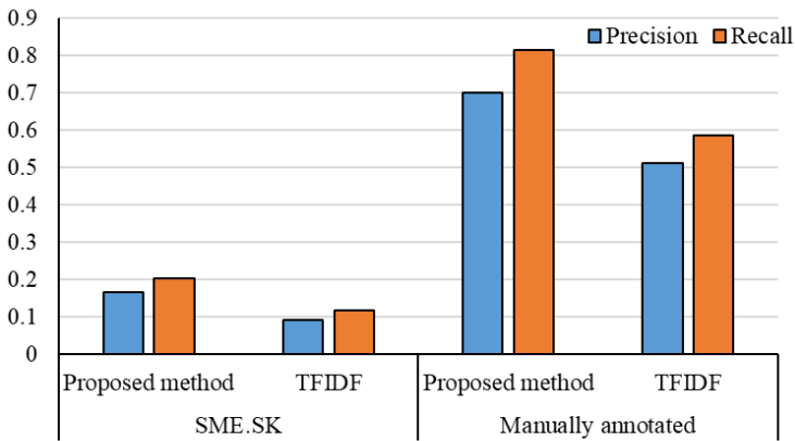
Fig. 25. The visualized results for the study by Kompan and Bielíková [125].
