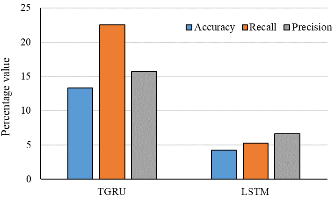
Fig. 10. Performance factors for comparing TGRU and LSTM with GRU
