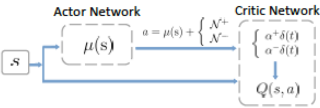
Fig. 23. Proposed model architecture [115]
