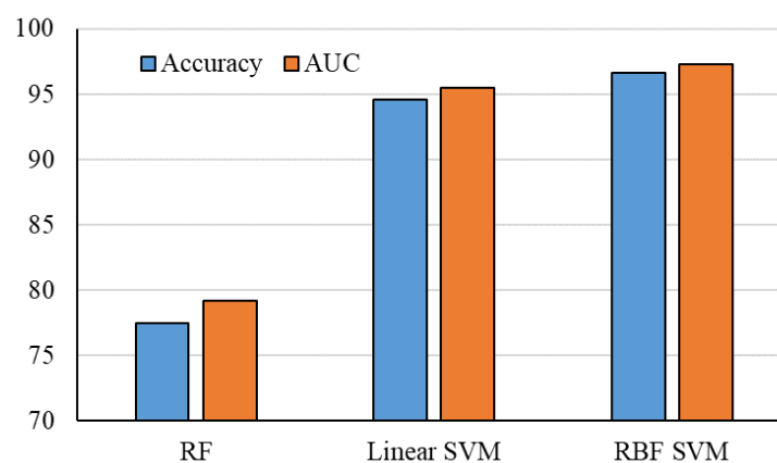
Fig. 21. Results for the study by Singh and Verma [31]
