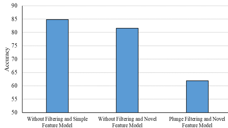
Fig. 11. Comparing accuracy values for the methods developed by Song et al [69]
