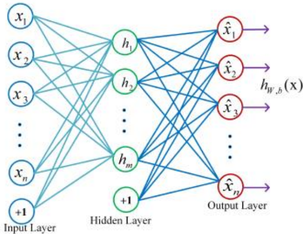
Figure 5. Simple architecture of Auto-Encoder [31]
