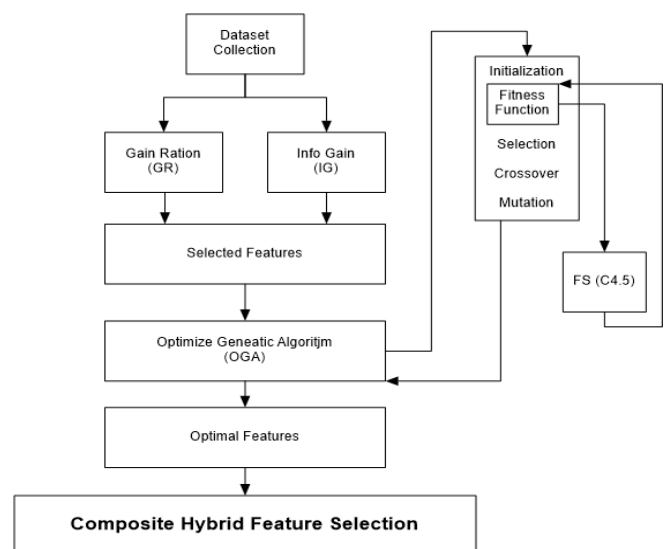
Fig.4 The proposed composite hybrid feature selection architecture
