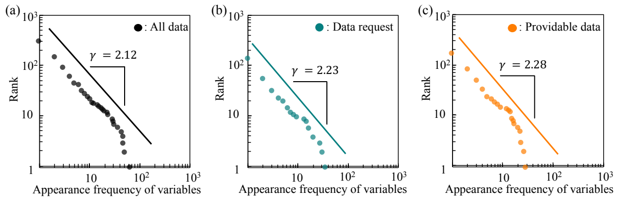
Figure 3. Distributions of the frequency of variables.
