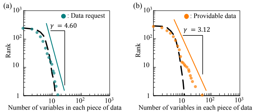
Figure 4. Distributions of the number of variables in each piece of data.
