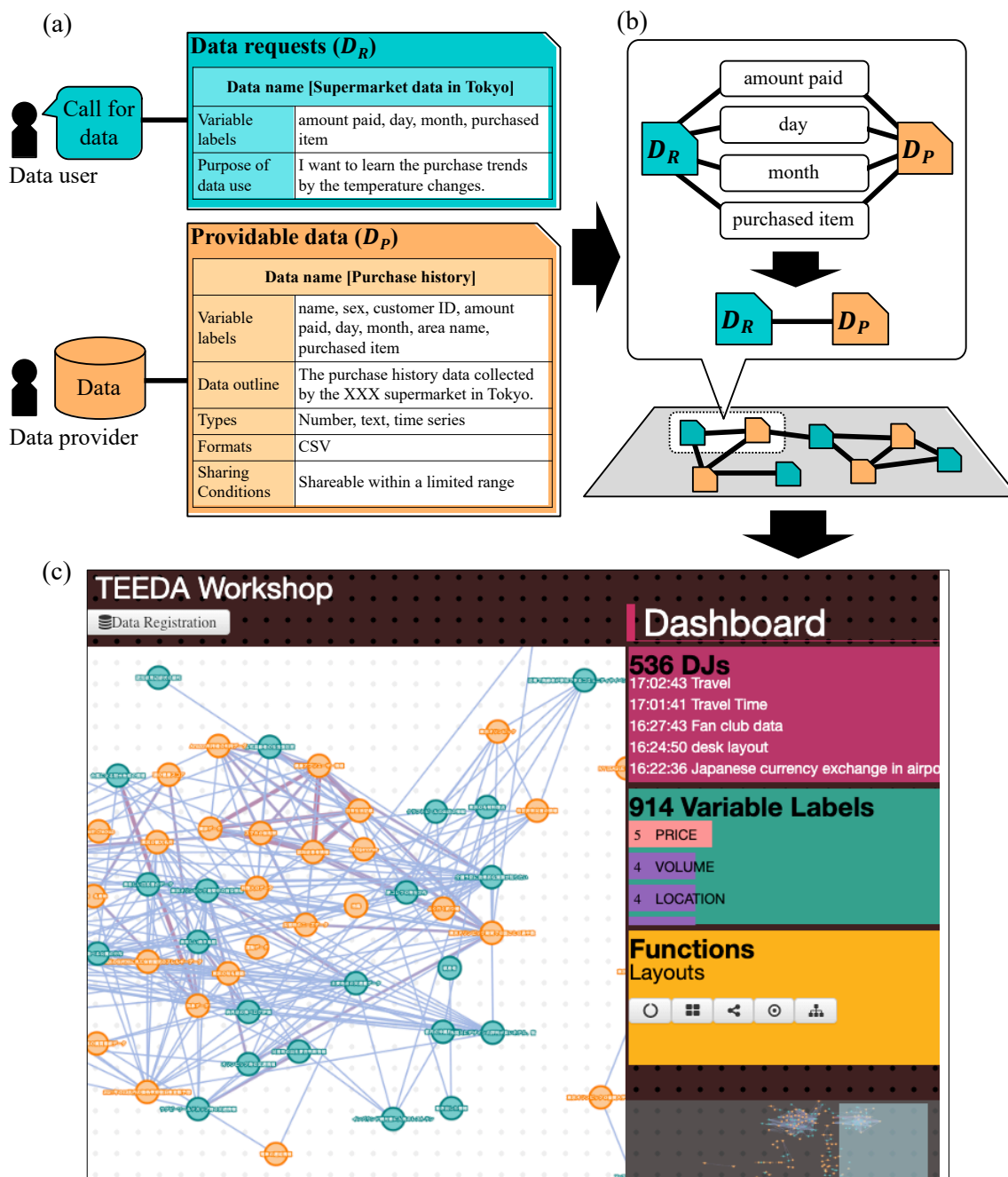
Figure 1. Process to collect and match data requests and providable data, and the TEEDA interface.
