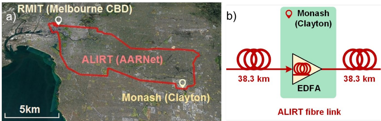
Supplementary Material Figure 2 – Field trial test link. a) Layout of the field trial link, linking RMIT and Monash labs via AARNet's fibre network, with route overlaid on Google Maps (red). Projection of the path of the installed fibre cabling onto a composite aerial image of the greater Melbourne metropolitan area (image courtesy of Google Maps). The fibre route included a mix of aerial and sub-surface fibres, comprising both OS1 and OS2 standard cables, and was provided by AARNet as part of the ALIRT project. b) Simplified schematic of fibre link, two 38.3 km fibre spans running along the same path with a remote EDFA at the Monash labs.
