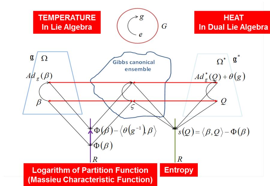
Figure 2. Souriau Model of Lie Groups Thermodynamics.
