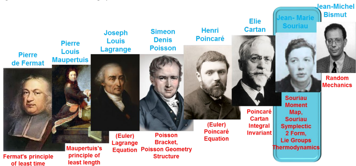
Figure 2. Jean-Marie Souriau contribution in the domain of Calculus of Variations.
