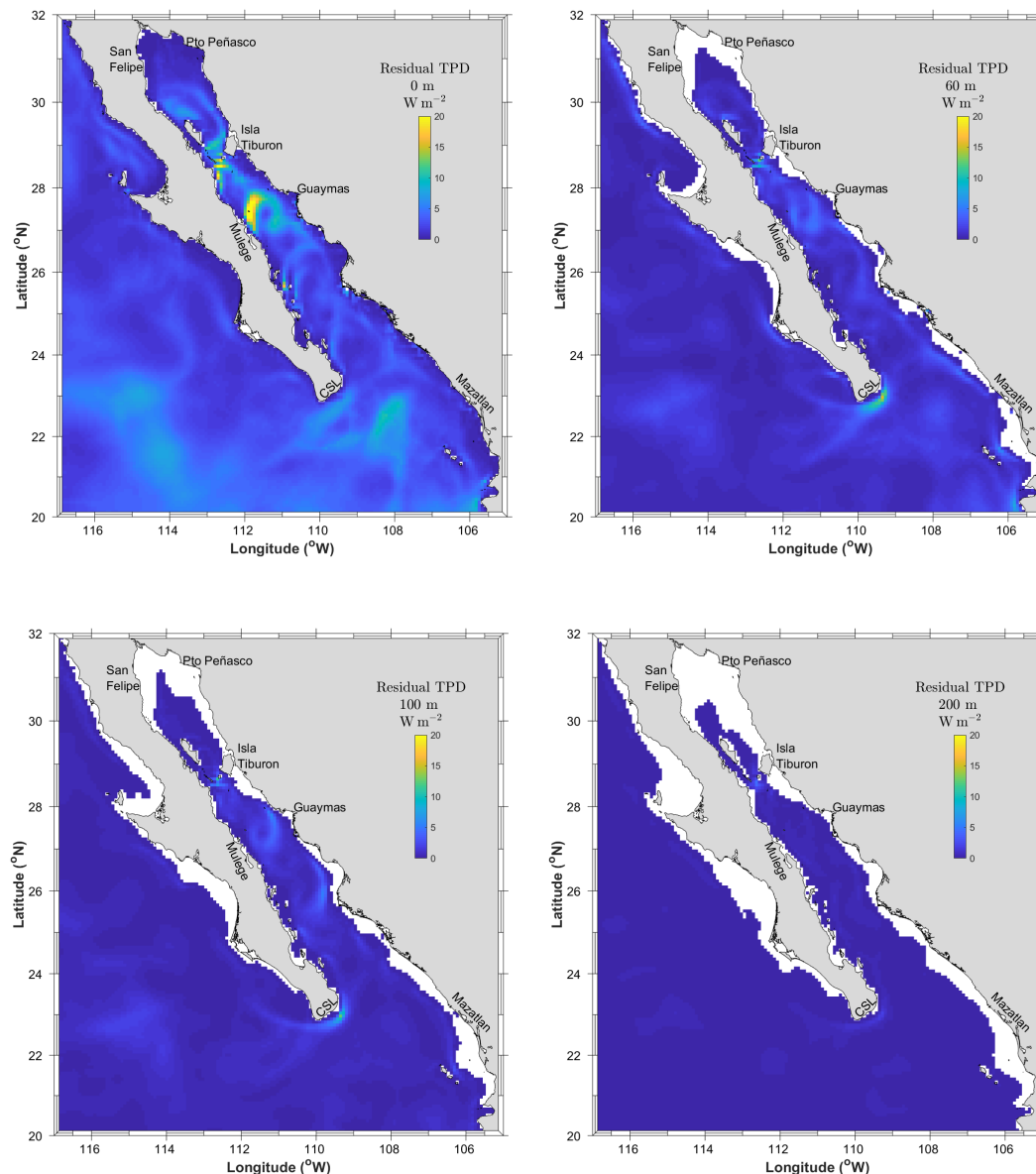
Figure 8. Residual \overline{TPD} at (a) 0 m, (b) 60 m, (c) 100 m, and (d) 200 m below Mean Sea Level.
