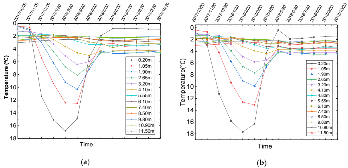
Figure 7. Ground temperature–time curve at different test sites: (a) test site 1; (b) test site 2.
