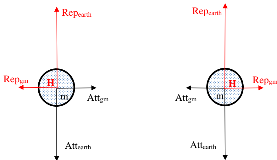
Figure. 1. Two air molecules with mass m and thermal energy H . Each molecule experiences gravitational attraction and repulsive forces from the other gas molecule ( Att_{gm} and Rep_{gm} ) as well as from the earth ( Rep_{earth} and Att_{earth} )
