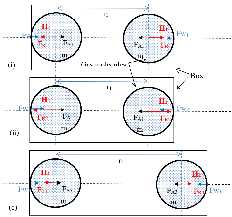
Figure. 5 Two air molecules under change of thermal energy (i) Temperature in the system is T_1 and the distance between them is r_1 . External pressure F_{w1} is applied for the equilibrium (ii) Temperature increases from T_1 to T_2 ( T_1 < T_2 ). Two molecules are at temperature T_2 but the distance, r_1 between them keep constant by applying an external pressure F_{w2} . (iii) Two molecules undergo isothermal expansion. Distance between molecules increases from r_1 to r_3 ( r_3 > r_1 ) until pressure becomes F_{w1}
