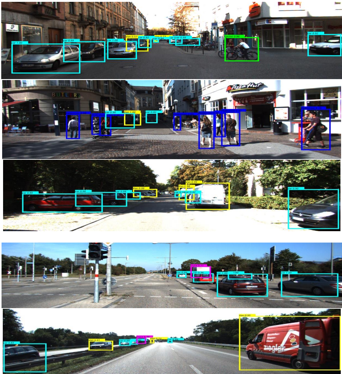
Figure 17: Obstacle detection has also been done using the YOLOv3 algorithm on the images obtained from real driving
