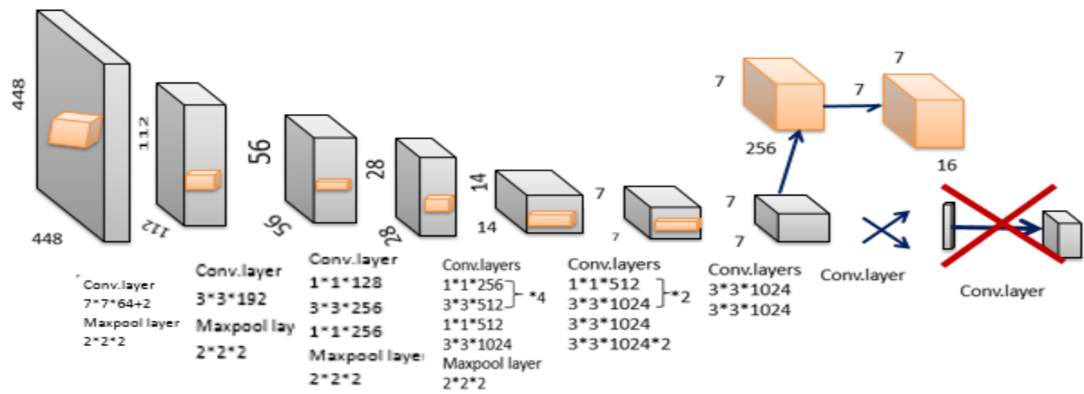
Figure 6: YOLOv3
