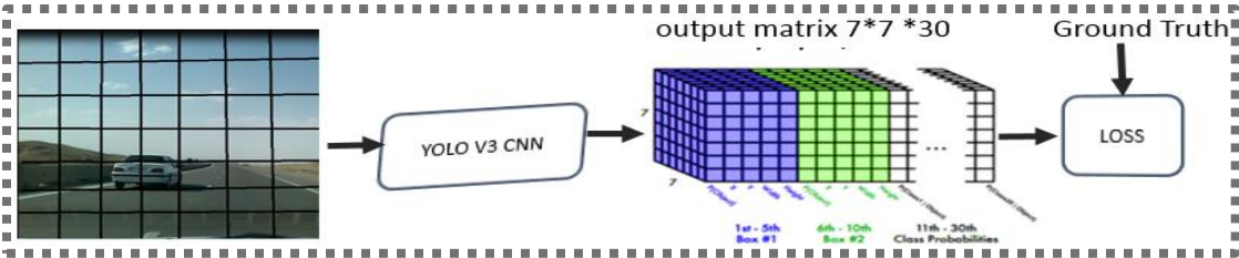
Figure 8: Overall structure of the YOLO system along with the input and the output
