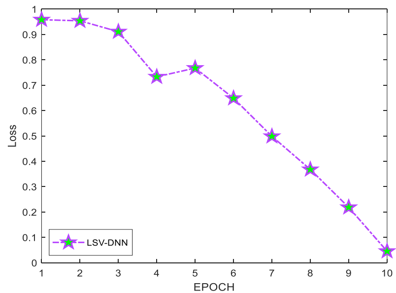
Figure 24: Loss over epochs
