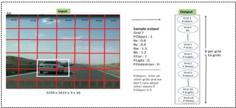
Figure 10: Boxes, input, and output of the YOLO architecture
