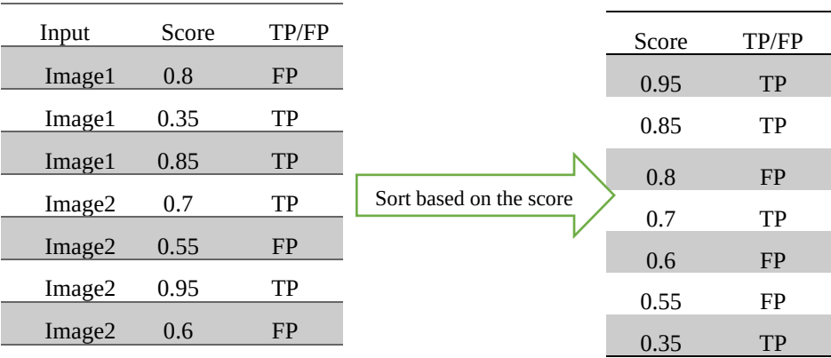
Figure 22: Sorting the scores of detected bboxes
