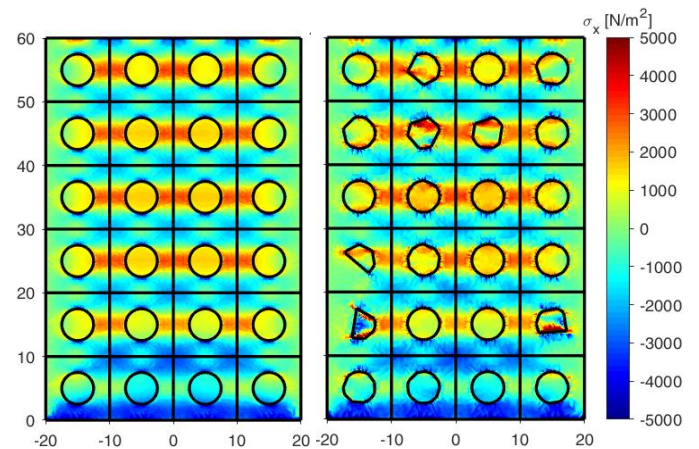
Fig. 25 \sigma_x values with round inclusions ( |\sigma_x|_{\max} = 6.541 \text{ kN/m}^2 , left) and irregular random inclusions ( |\sigma_x|_{\max} = 42.831 \text{ kN/m}^2 , right)
