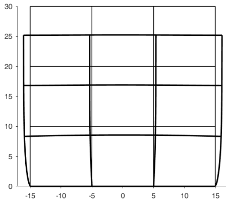
Fig. 12 deformed configuration of the 3 \times 3 array without inclusions (displacement amplification factor: k = 400 ).
