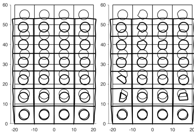
Fig. 23 deformed configurations for the 6 \times 4 arrays with round inclusions (left) and irregular random inclusions (right): amplification factor k = 400
