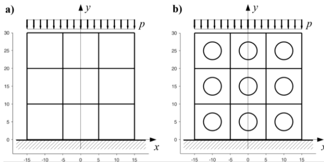
Fig. 1 loading conditions for the 3 \times 3 arrays: a) without inclusion and b) with round inclusions (linear measurements in mm)
