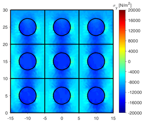
Fig. 14 \sigma_y values: inclusions with 35 sides, |\sigma_y|_{\max} = 18.034 \text{ kN/m}^2
