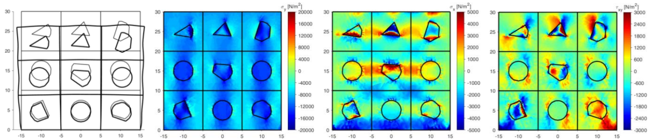
Fig. 20 first set of inclusions: amplification factor k = 400 , |\sigma_y|_{\max} = 51.760 \text{ kN/m}^2 , |\sigma_x|_{\max} = 49.073 \text{ kN/m}^2 , |\tau_{xy}|_{\max} = 19.188 \text{ kN/m}^2
