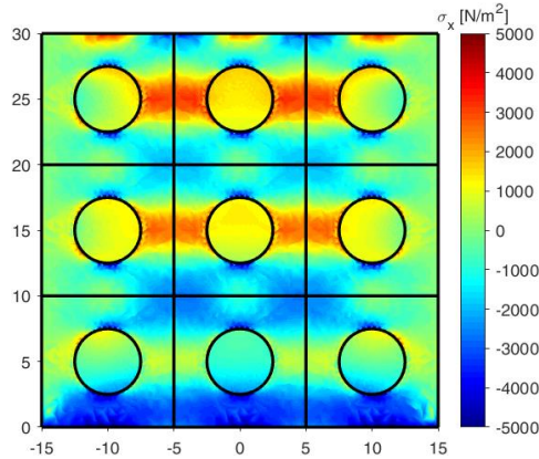
Fig. 8 \sigma_x values with round inclusions: |\sigma_x|_{\max} = 6.346 \text{ kN/m}^2
