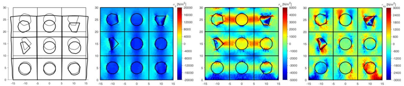
Fig. 21 second set of inclusions: amplification factor k = 400 , |\sigma_y|_{\max} = 77.917 \text{ kN/m}^2 , |\sigma_x|_{\max} = 56.033 \text{ kN/m}^2 , |\tau_{xy}|_{\max} = 24.422 \text{ kN/m}^2
