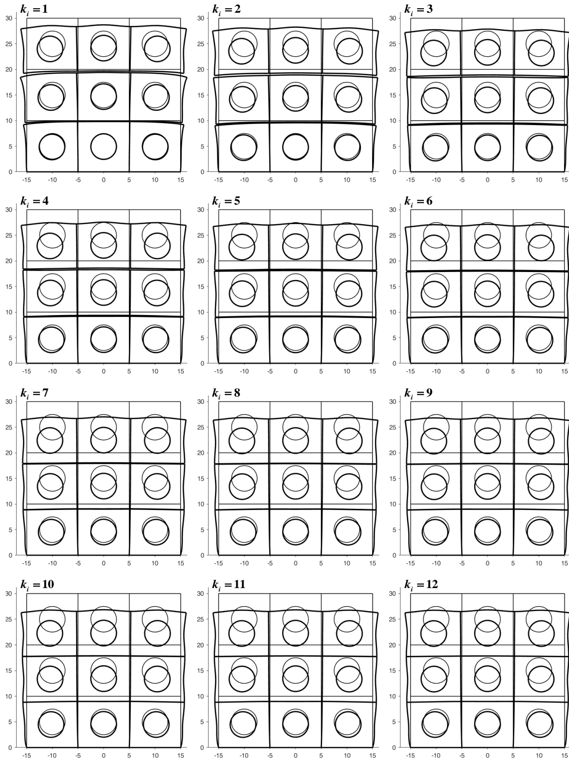
Fig. 3 deformed configurations provided by the k_i -th top-to-bottom-to-top iteration, for 1 \leq k_i \leq 12 (thin line: undeformed configurations; thick line: deformed configurations, amplification factor of the displacements: k = 400 ) sides (where the displacements are known). In the iteration performs a new left-to-right-to-left procedure on the n_c
