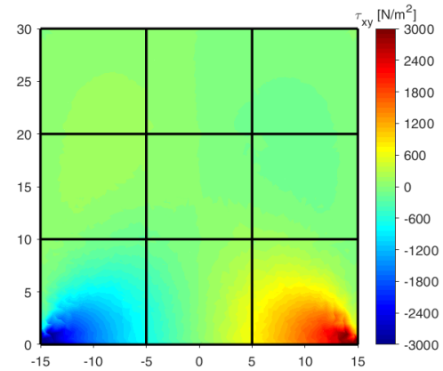
Fig. 6 shear stress \tau_{xy} with no inclusions: |\tau_{xy}|_{\max} = 3.575 \text{ kN/m}^2
