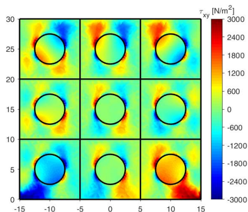
Fig. 9 \tau_{xy} values with round inclusions: |\tau_{xy}|_{\max} = 3.312 \text{ kN/m}^2
