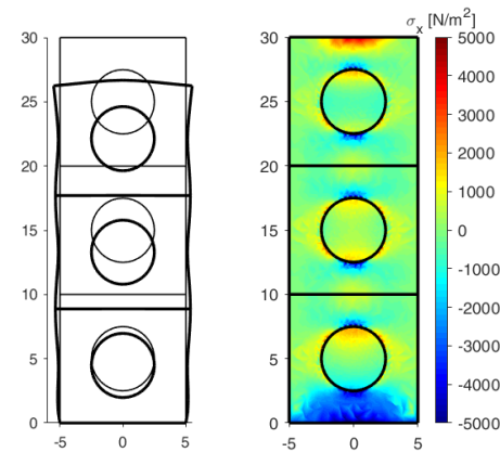
Fig. 10 deformed configuration and normal stress \sigma_x for a 3 \times 1 array with round inclusions and constrained displacements on the base (displacement amplification factor: k = 400 , distributed compressive axial load p = p_y = 10 \text{ kN/m}^2 , |\sigma_x|_{\max} = 5.996 \text{ kN/m}^2 )
