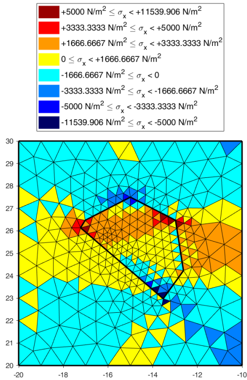
Fig. 28 discrete stress field \sigma_x for the (4,1) entry of the 6 \times 4 array with irregular random inclusions in Fig. 25
