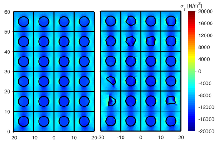
Fig. 24 \sigma_y values with round inclusions ( |\sigma_y|_{\max} = 16.579 \text{ kN/m}^2 , left) and irregular random inclusions ( |\sigma_y|_{\max} = 97.797 \text{ kN/m}^2 , right)
