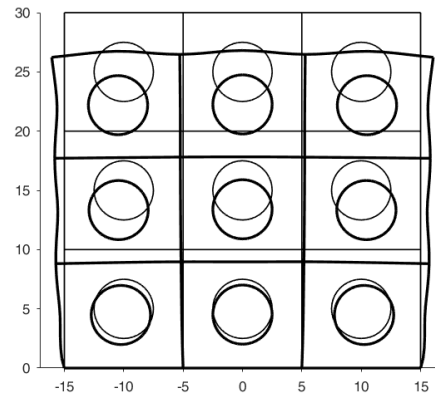
Fig. 11 deformed configuration of the 3 \times 3 array with round inclusions (displacement amplification factor: k = 400 ).
