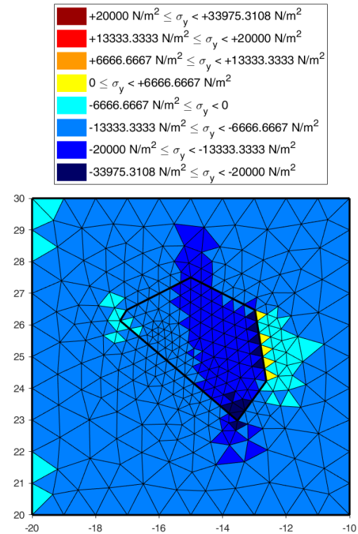
Fig. 27 discrete stress field \sigma_y for the (4,1) entry of the 6 \times 4 array with irregular random inclusions in Fig. 24
