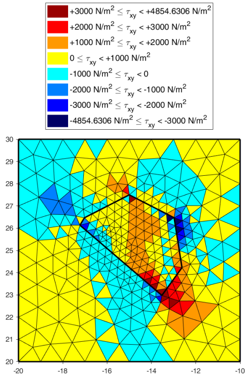
Fig. 29 discrete stress field \tau_{xy} for the (4,1) entry of the 6 \times 4 array with irregular random inclusions in Fig. 26
