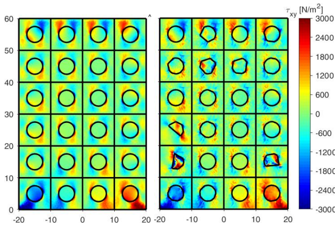
Fig. 26 \tau_{xy} values with round inclusions ( |\tau_{xy}|_{\max} = 3.539 \text{ kN/m}^2 , left) and irregular random inclusions ( |\tau_{xy}|_{\max} = 20.156 \text{ kN/m}^2 , right)
