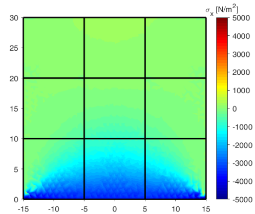
Fig. 5 normal stress \sigma_x with no inclusions: |\sigma_x|_{\max} = 5.413 \text{ kN/m}^2
