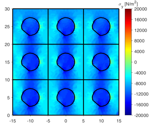
Fig. 17 \sigma_y values: inclusions with 25 sides and a greater degree of irregularity than Fig. 16, |\sigma_y|_{\max} = 22.876 \text{ kN/m}^2
