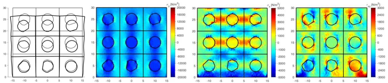
Fig. 22 third set of inclusions: amplification factor k = 400 , |\sigma_y|_{\max} = 39.958 \text{ kN/m}^2 , |\sigma_x|_{\max} = 17.624 \text{ kN/m}^2 , |\tau_{xy}|_{\max} = 6.391 \text{ kN/m}^2
