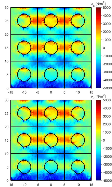
Fig. 18 \sigma_x values: inclusions with 25 sides and degree of irregularity that increases from the upper 3 \times 3 array ( |\sigma_x|_{\max} = 6.510 \text{ kN/m}^2 ) to the lower 3 \times 3 array ( |\sigma_x|_{\max} = 6.860 \text{ kN/m}^2 )
