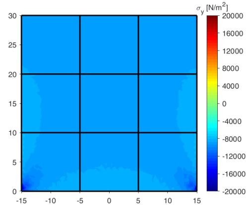
Fig. 4 normal stress \sigma_y with no inclusions: |\sigma_y|_{\max} = 18.406 \text{ kN/m}^2
