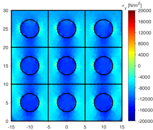
Fig. 16 \sigma_y values: inclusions with 25 sides, |\sigma_y|_{\max} = 18.840 \text{ kN/m}^2
