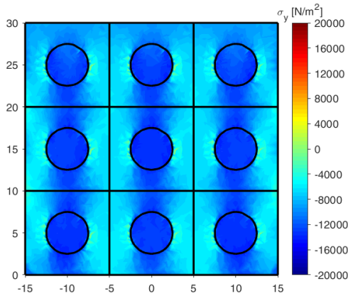
Fig. 15 \sigma_y values: inclusions with 30 sides, |\sigma_y|_{\max} = 18.681 \text{ kN/m}^2
