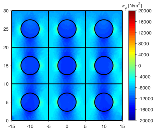
Fig. 7 \sigma_y values with round inclusions: |\sigma_y|_{\max} = 16.178 \text{ kN/m}^2
