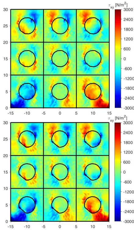
Fig. 19 \tau_{xy} values: inclusions with 25 sides and degree of irregularity that increases from the upper 3 \times 3 array ( |\tau_{xy}|_{\max} = 3.733 \text{ kN/m}^2 ) to the lower 3 \times 3 array ( |\tau_{xy}|_{\max} = 5.248 \text{ kN/m}^2 )
