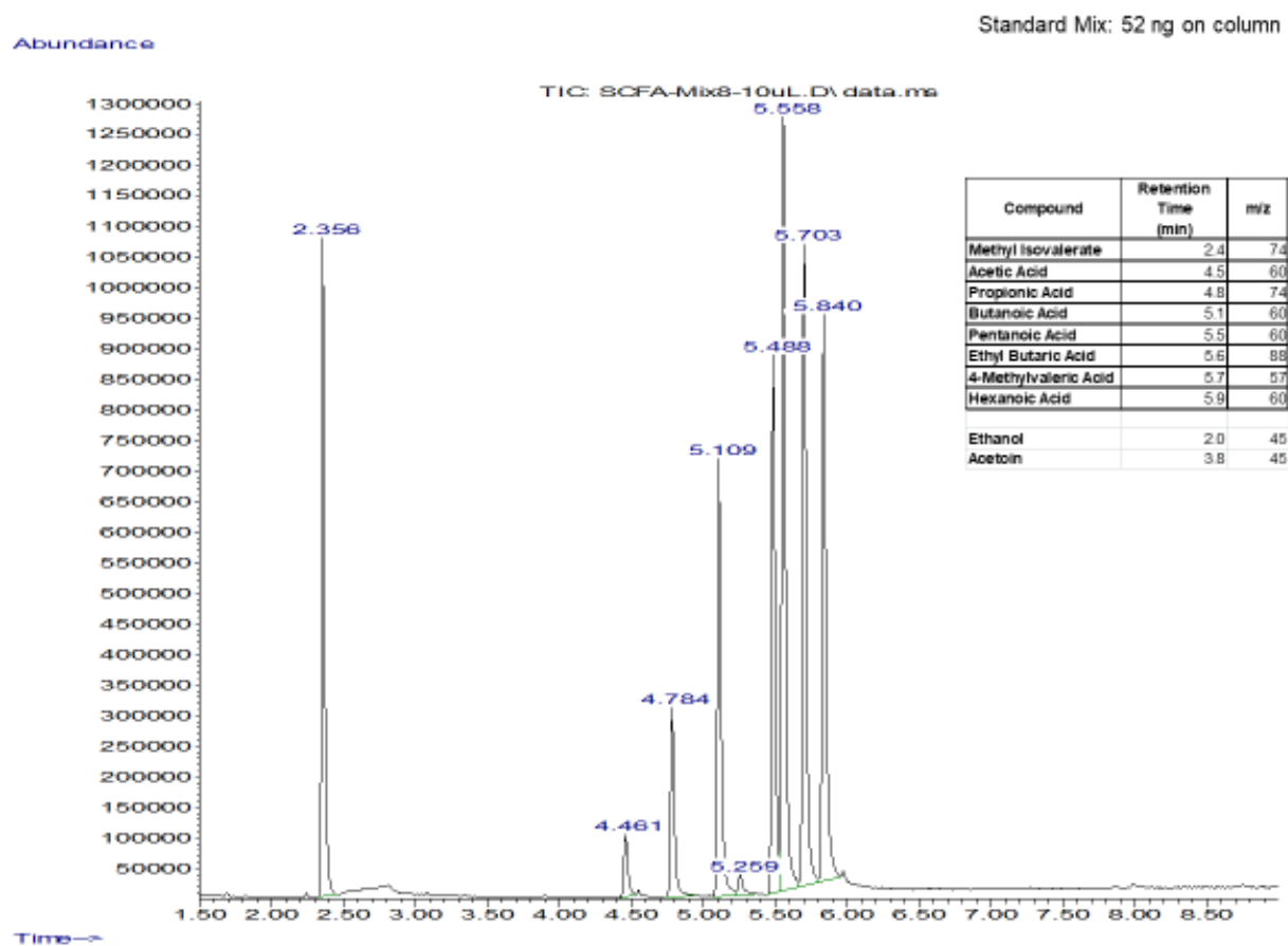
Figure 3. Headspace-GCMS total ion chromatogram of standard mix (5 SCFA and 3 analogs) from a 52 ng injection of each component on column. Inset table provided as a guide showing the retention times and identifying m/z value for each component.
