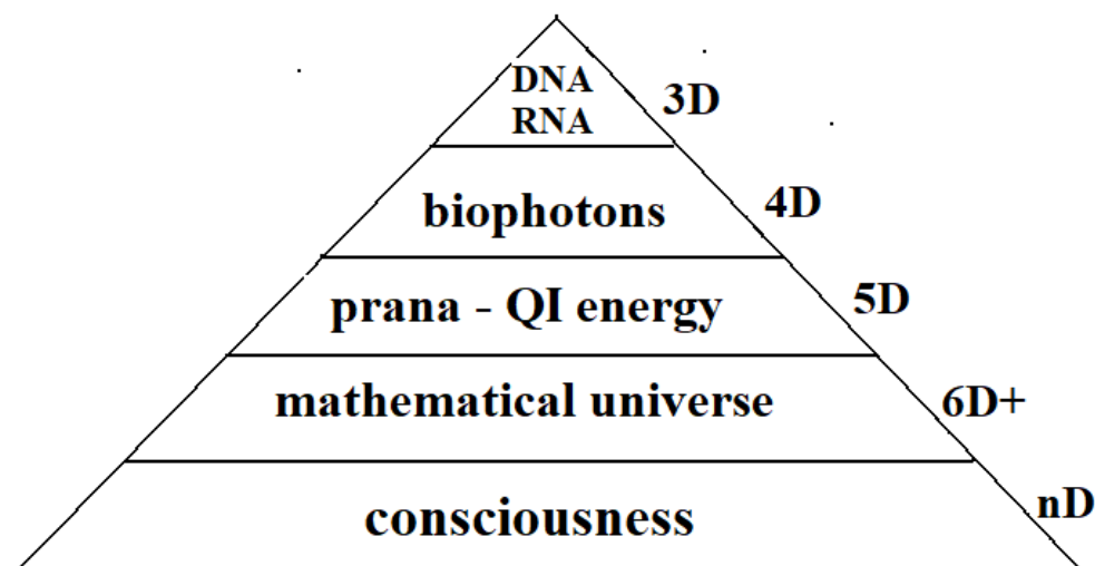
Figure 2: Life-information system in \mathbb{C}^n SQS that exists in the entire universe.
