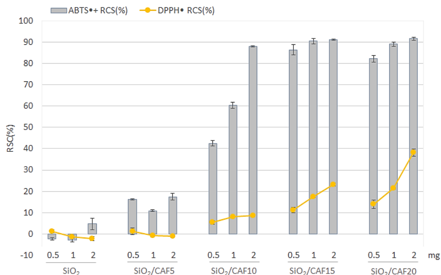
Figure 5. Radical Scavenging Capacity (RSC, %) towards DPPH• and ABTS•+ of SiO 2 and hybrid materials differing for the amount of caffeic acid (CAF5=caffeic acid 5 wt%; CAF10=caffeic acid 10 wt%; CAF15=caffeic acid 15 wt%; CAF20=caffeic acid 20 wt%). Values, reported as percentage vs. a blank, are the mean \pm SD of measurements carried out on three samples (n = 3) analyzed three times.
