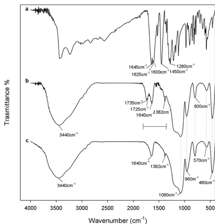
Figure 2. FT-IR spectra of: a) pure caffeic acid; b) \text{SiO}_2 /caffeic acid 20 wt% hybrid material; c) pure \text{SiO}_2
