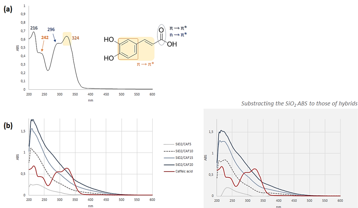
Figure 3. UV-Vis spectra of (a) pure caffeic acid dissolved in EtOH at a molar concentration of 3.5 \cdot 10^{-5} mol L -1 ; (b) hybrid materials differing for the amount of caffeic acid (CAF5=caffeic acid 5 wt%; CAF10=caffeic acid 10 wt%; CAF15=caffeic acid 15 wt%; CAF20=caffeic acid 20 wt%). In the grey box UV-Vis spectra were reported after subtracting the SiO 2 absorbance (ABS) values to those of each hybrid. Red lines refer to pure caffeic acid.
