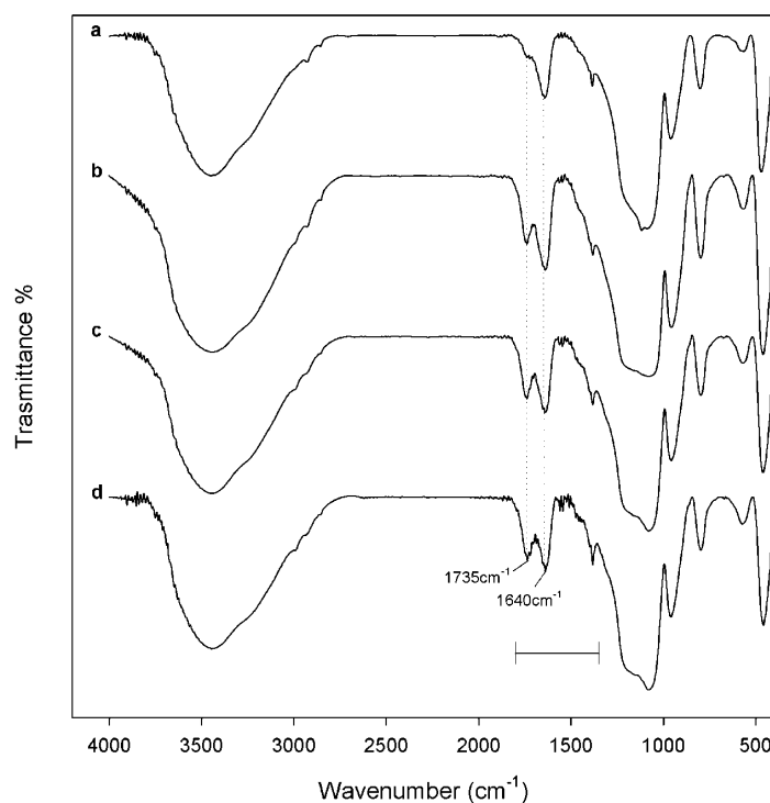
Figure 3. FT-IR spectra of synthesized materials: a) SiO 2 /caffeic acid 5 wt%; b) SiO 2 /caffeic acid 10 wt%; c) SiO 2 /caffeic acid 15 wt%; d) SiO 2 /caffeic acid 20 wt%. Spectra were vertically shifted to help in the comparison.
