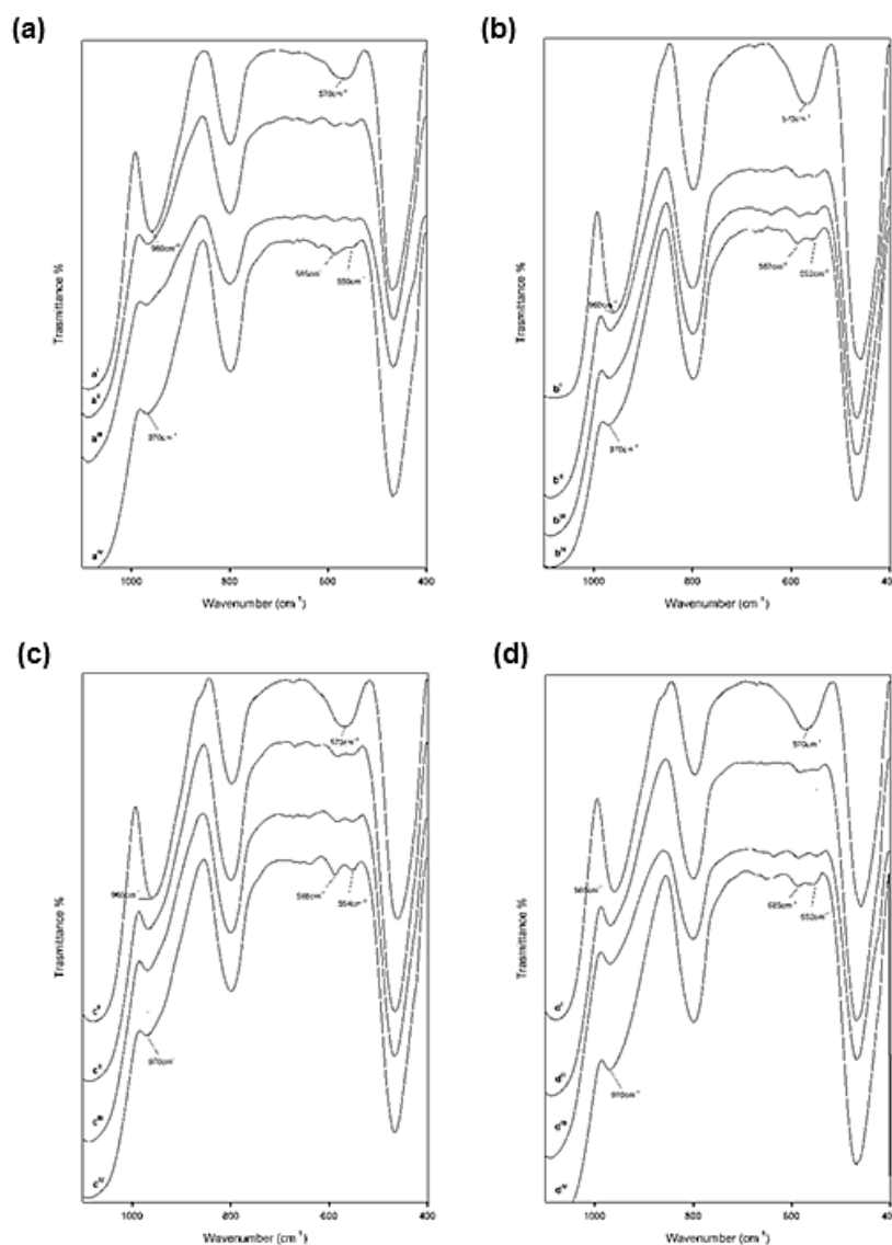
Figure 4. FT-IR spectra of (a) SiO 2 /caffeic acid 5 wt% ; (b) SiO 2 /caffeic acid 10 wt%; (c) SiO 2 /caffeic acid 15 wt%; (d) SiO 2 /caffeic acid 20 wt%. For each sample spectra acquired before exposure to SBF (I) were compared to those recorded after 7, 14 and 21 days of exposure to SBF (II-IV). Spectra were vertically shifted to help in the comparison.
