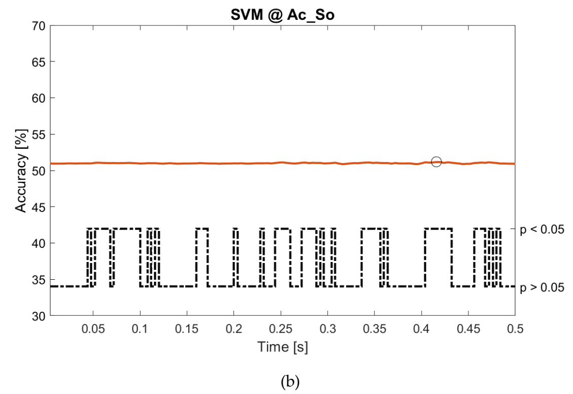
Figure 6. Spectral dynamic features. Accuracy (mean value, coloured line; standard deviation, shaded line) and p-values (black dotted line) in Ac_So group for LDA (a) and SVM (b) classifiers.
