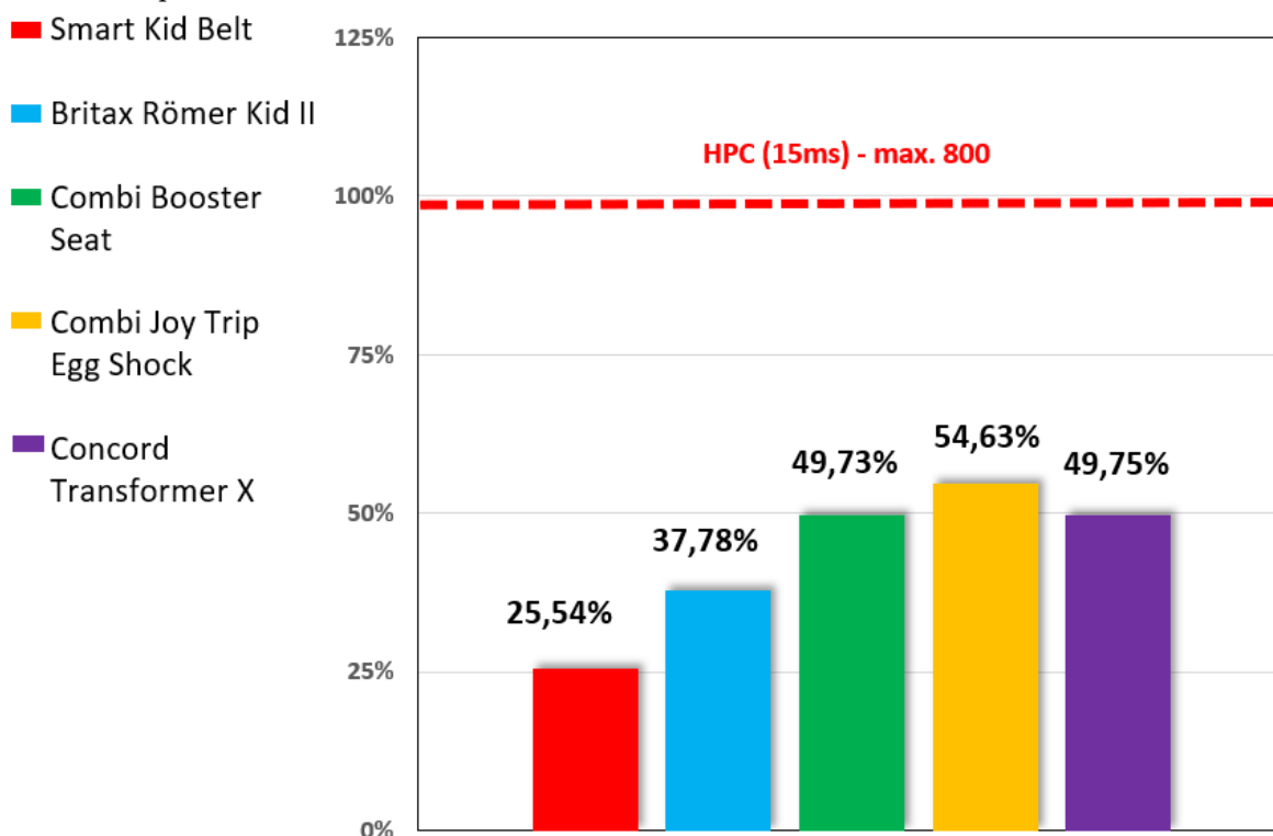
Figure 6. Head Performance Critrion for all tested devices regarding to the maximum limit.
