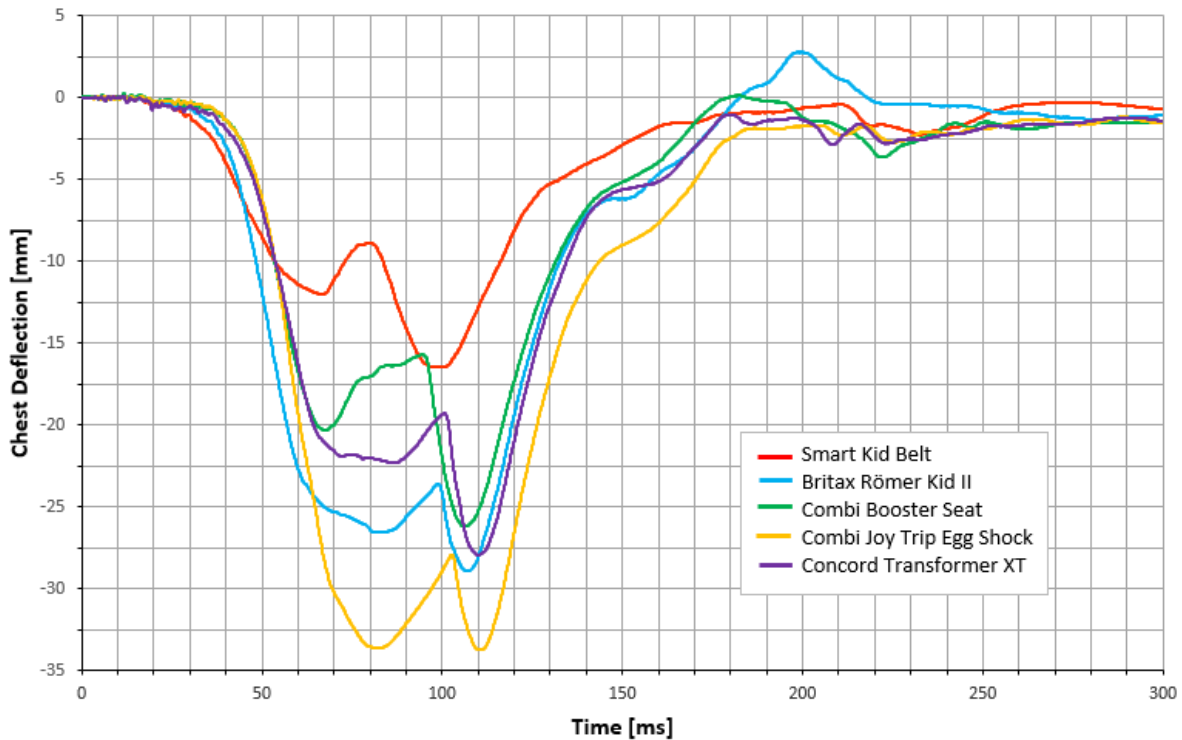
Figure 8. Chest deflection-for all tested devices.
