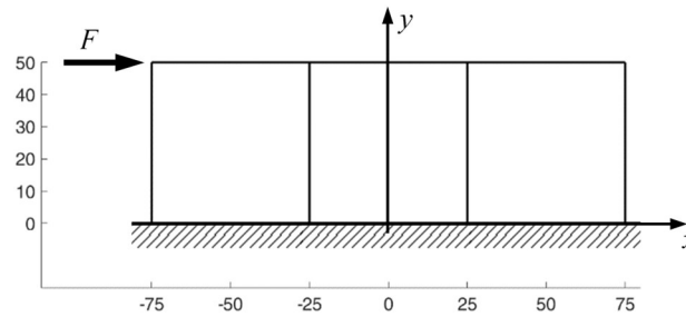
Figure 14. Geometry of a two-dimensional domain consisting of 1 row of 3 square elements (linear measurements in mm).
