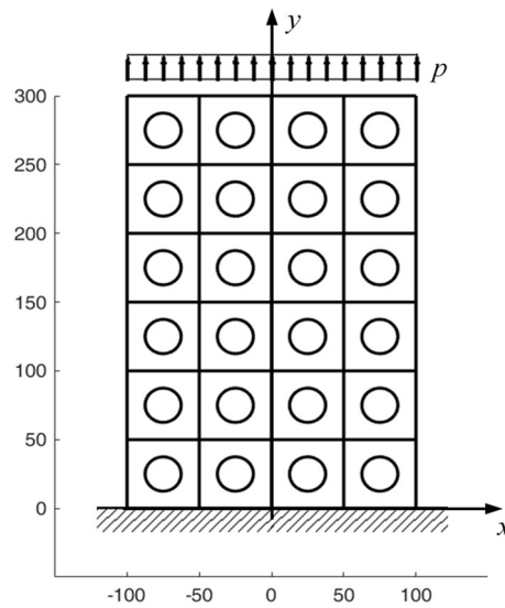
Figure 26. Geometry and loading condition of the 6 \times 4 array with round inclusions (linear measurements in mm).
