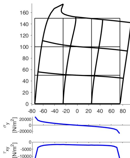
Figure 19. Deformed configurations of the 9 discrete elements and stress analysis on the lower constrained sides, after 15 top-to-bottom-to-top stabilization cycles on the rows (thin line: undeformed configurations; thick line: deformed configurations, amplification factor of the displacements: k = 200 ).
