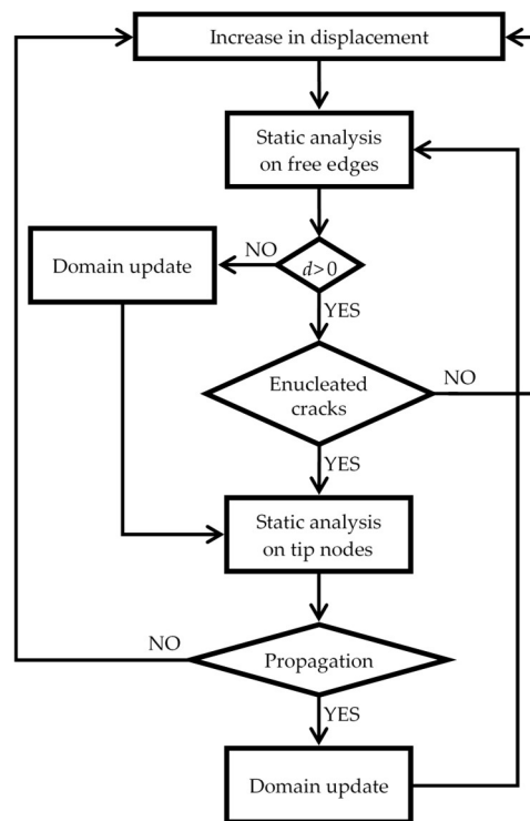
Figure 32. Flow chart of a CM code for the analysis of crack propagation in displacement control.
