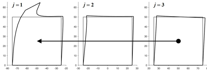
Figure 16. First iteration from right to left: the j -th element generates the displacements on the right side of the (j-1) -th element, with j=3,2 (thin line: undeformed configurations; thick line: deformed configurations, amplification factor of the displacements: k=200 ).
