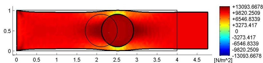
Figure 28. CM static analysis: normal stresses \sigma_x plotted on the deformed configuration (thin line: undeformed configuration, thick line: deformed configuration, amplification factor of the displacements: k = 500 ). [45]
