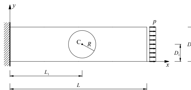
Figure 27. Geometry and loading condition of the elastic cantilever beam with round inclusion. [45]
