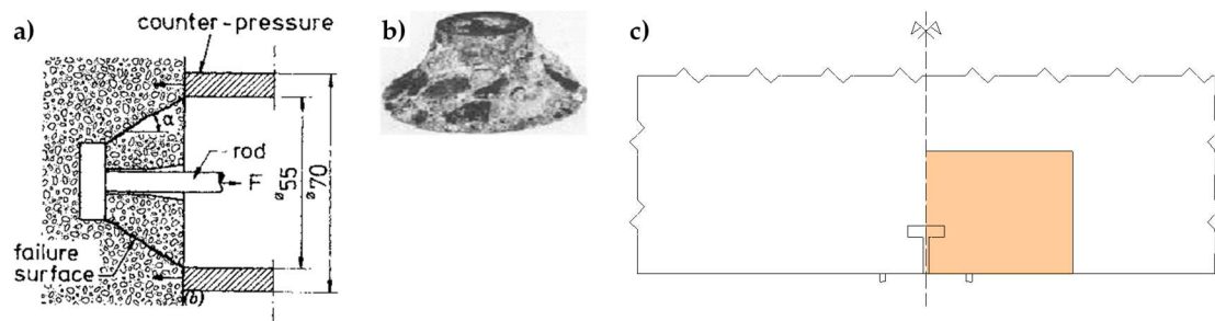
Figure 2. The Lok-Test: a) Geometric characteristics of the insert and counter-pressure for pullout test; b) Shape of the extracted portion in concrete solids; c) Shape of the modeled domain.
