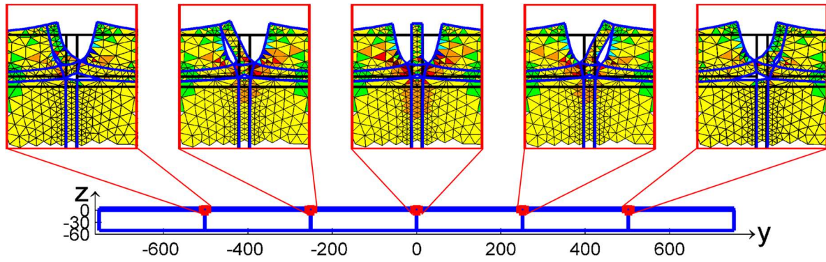
Figure 6. Details of detachments on the tiles joints for temperature variation.
