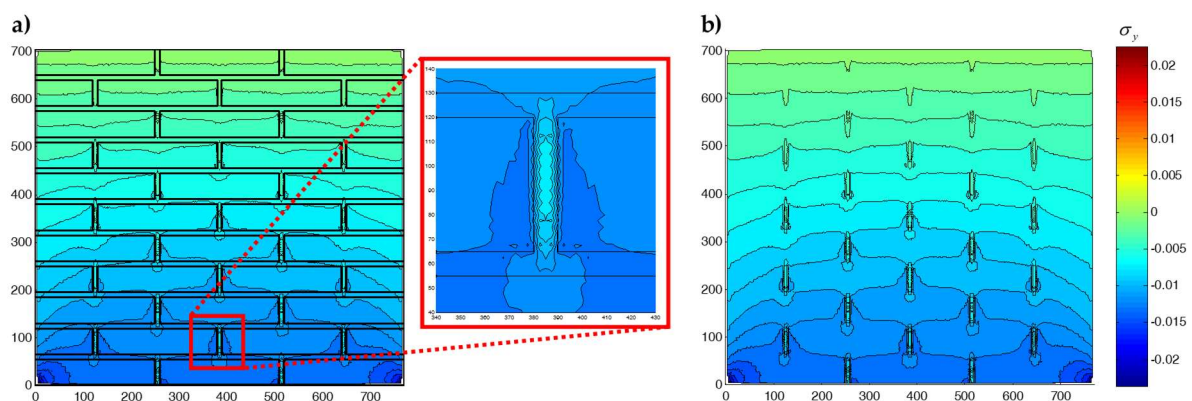
Figure 1. Isolines of the normal stress \sigma_y (the y -axis runs vertically): a) with and b) without the arrangement of the bricks in the foreground (stress values in \text{N/mm}^2 and linear measurements in mm).
