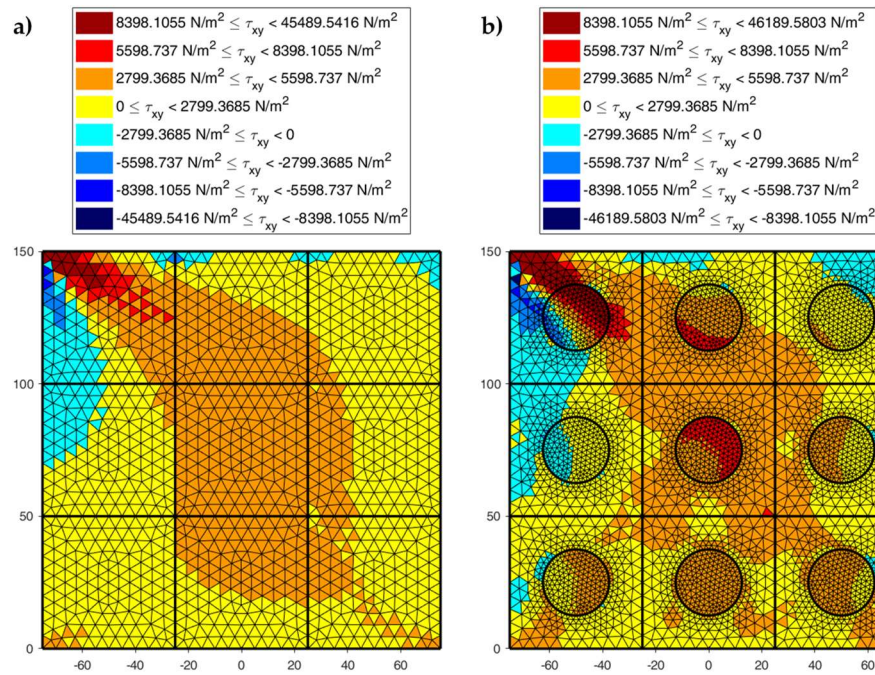
Figure 24. Shear stresses \tau_{xy} in the discrete elements of a 3 \times 3 array subjected to shear load: a) Without inclusions and b) With round inclusions, stiffer than the matrix.
