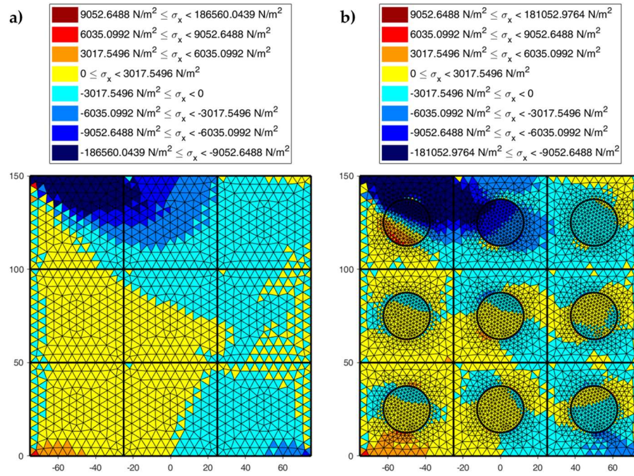
Figure 23. Normal stresses \sigma_x in the discrete elements of a 3 \times 3 array subjected to shear load: a) Without inclusions and b) With round inclusions, stiffer than the matrix.
