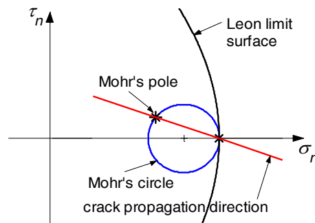
Figure 11. Limit domain of Leon in the Mohr/Coulomb plane.
