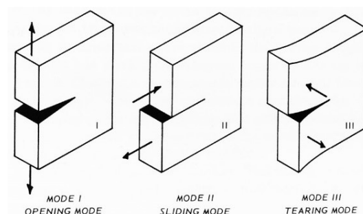
Figure 7. The three modes of propagation in fracture mechanics.
