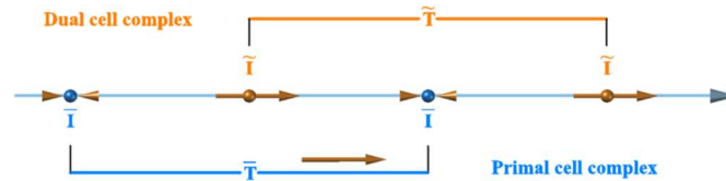
Figure 34. Time elements in the primal and dual cell-complexes.
