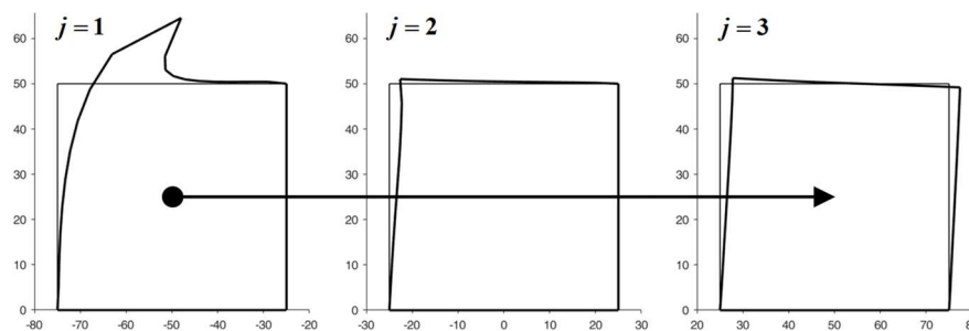
Figure 15. First iteration from left to right: the j -th element generates the forces on the left side of the (j+1) -th element, with j=1,2 (thin line: undeformed configurations; thick line: deformed configurations, amplification factor of the displacements: k = 200 ).
