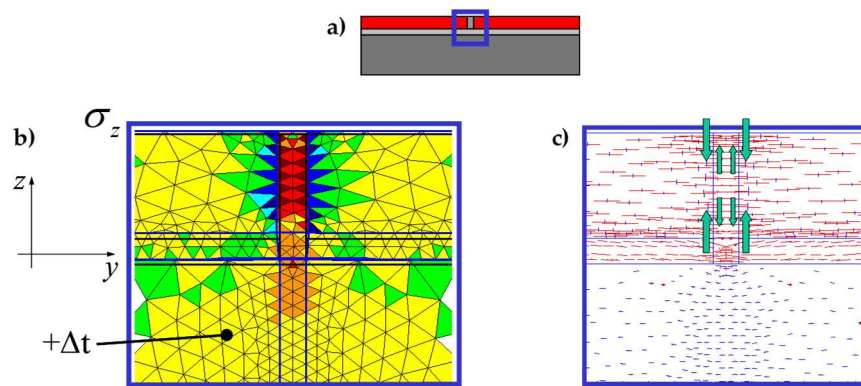
Figure 4. Modeling of joints in radiant heat floors: a) Detail of the modeled area; b) Field of the vertical stresses; b) Principal directions of stress.
