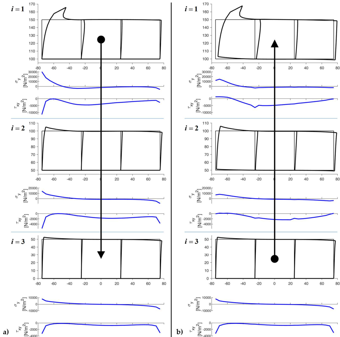
Figure 18. Deformed configurations of the stabilized rows and stress analysis on the constrained sides for the first top-to-bottom-to-top stabilization cycle on the rows: a) in the first iteration from top to bottom, the i -th row generates the forces on the upper sides of the (i+1) -th row, with i=1,2 ; b) in the first iteration from bottom to top, the i -th row generates the displacements on the lower sides of the (i-1) -th row, with i=3,2 (thin line: undeformed configurations; thick line: deformed configurations, amplification factor of the displacements: k=200 ).
