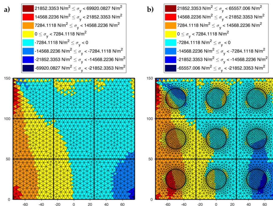
Figure 22. Normal stresses \sigma_y in the discrete elements of a 3 \times 3 array subjected to shear load: a) Without inclusions and b) With round inclusions, stiffer than the matrix.
