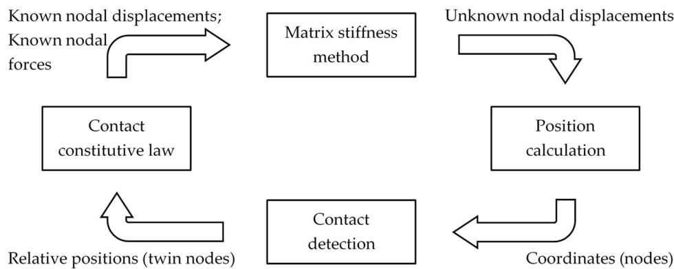
Figure 8. The DECM stabilization procedure to take into account both the compatibility and the equilibrium on the interfaces.
