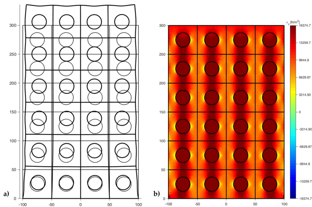
Figure 30. Elastic modeling of the 6 \times 4 array subjected to uniaxial traction: a) Deformed configuration (amplification factor of the displacements: k = 400 ) and b) Normal stresses \sigma_y .
