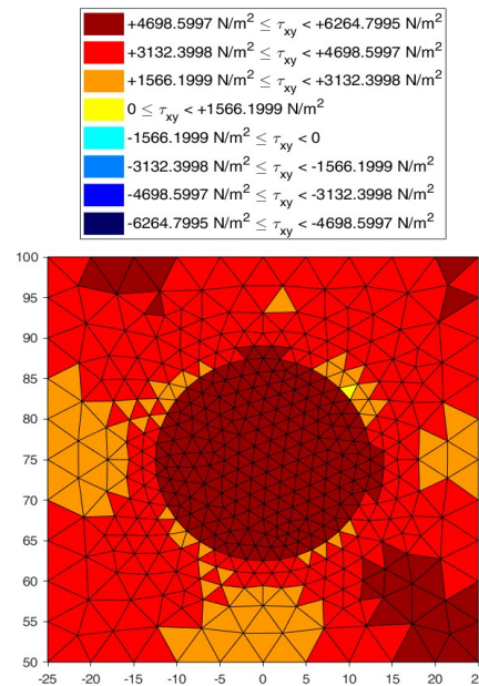
Figure 25. Detail of the shear stress \tau_{xy} for the discrete element i = 2, j = 2 (colors equally ranged between the extreme values of shear stress for the element).
