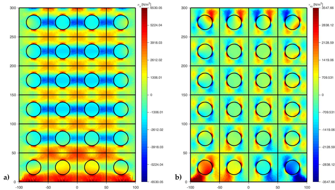
Figure 31. Stress fields in the 6 \times 4 array subjected to uniaxial traction: a) Normal stresses \sigma_x and b) Shear stresses \tau_{xy} .
