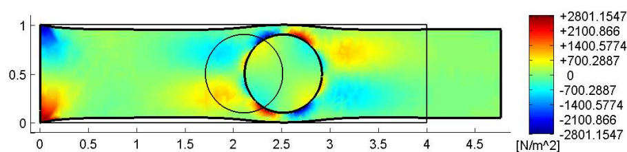
Figure 29. CM static analysis: shear stresses \tau_{xy} plotted on the deformed configuration (thin line: undeformed configuration, thick line: deformed configuration, amplification factor of the displacements: k = 500 ). [45]
