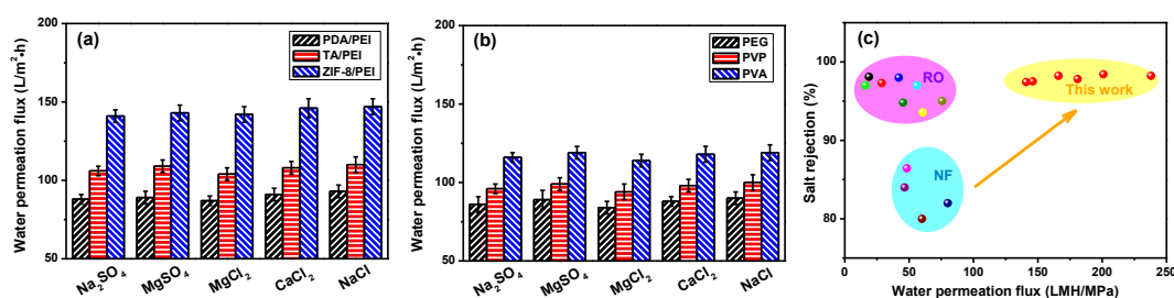
Figure 5. Water permeation flux of the as-prepared NF membranes with (a) the hydrophilic modified interlayers on the porous substrates or (b) the addition of macromolecular additives in the aqueous PIP solution (test conditions: inorganic salts concentration = 1000 mg/L, pH = 6.0, 25 °C, applied pressure = 0.6 MPa and cross-flow rate = 30 L/h) (c) the comparison of the NF performance with other thin-film composite membranes in the reported literature [39].
