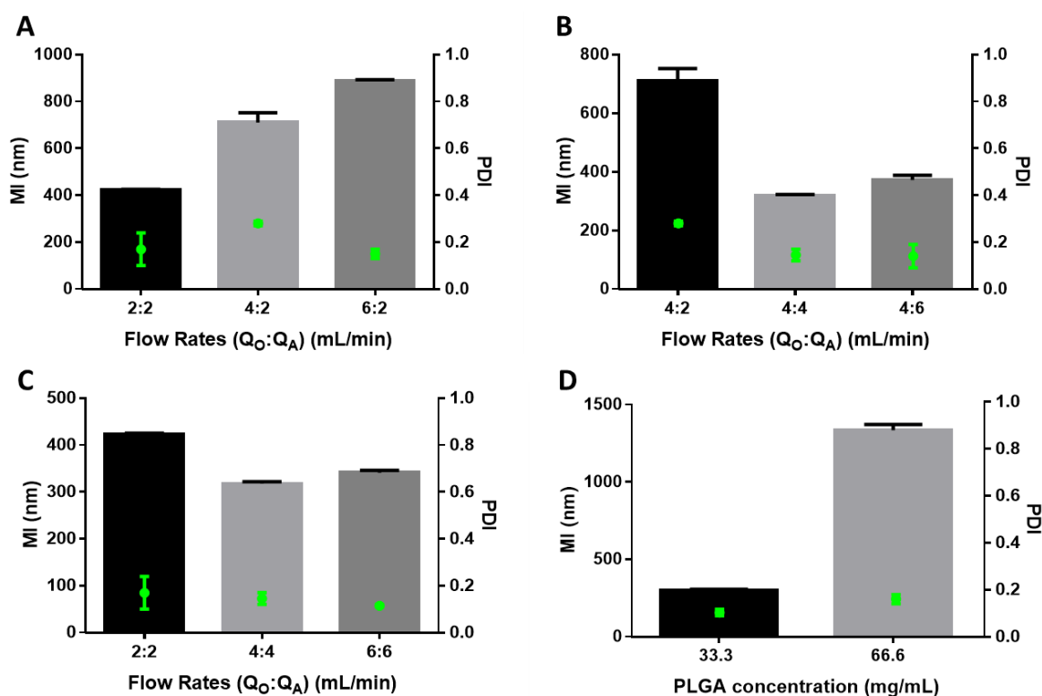
Figure 1. Influence of process and formulation parameters on the particle size. The variation of particle size at different flow rates for 33.3 mg/mL PLGA as organic phase and 1% PVA as aqueous phase (A-C). D) The influence of PLGA concentration on the particle size (organic:aqueous flow rate of 4:4 mL/min, 3% PVA as aqueous phase). (Bars: intensity-averaged particle size; Green dots: PDI).
