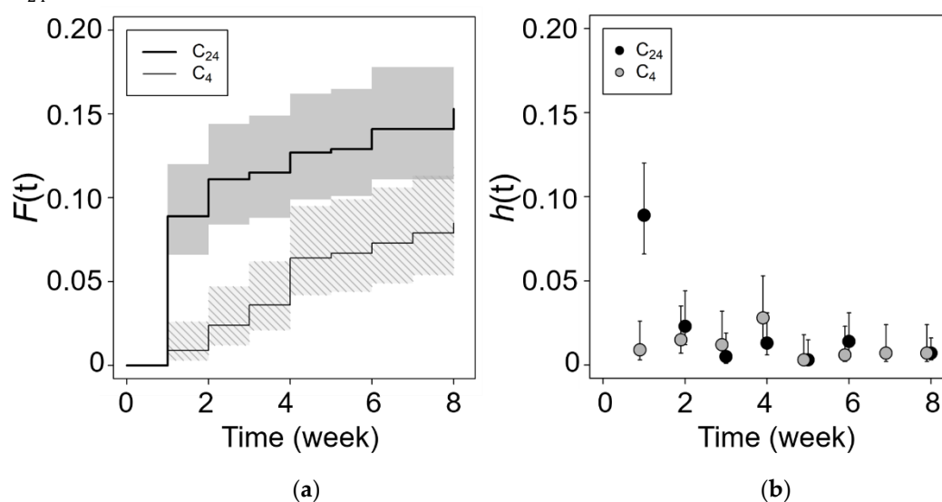
Figure 2. Germination test. Chilling treatments ( C_{24} and C_4 ) averaged over common salinity levels ( N_1 , N_{50} and N_{150} ), mean \pm 95% CI bands or bars for (a) germination probability, F(t) and (b) hazard rate, h(t) .
