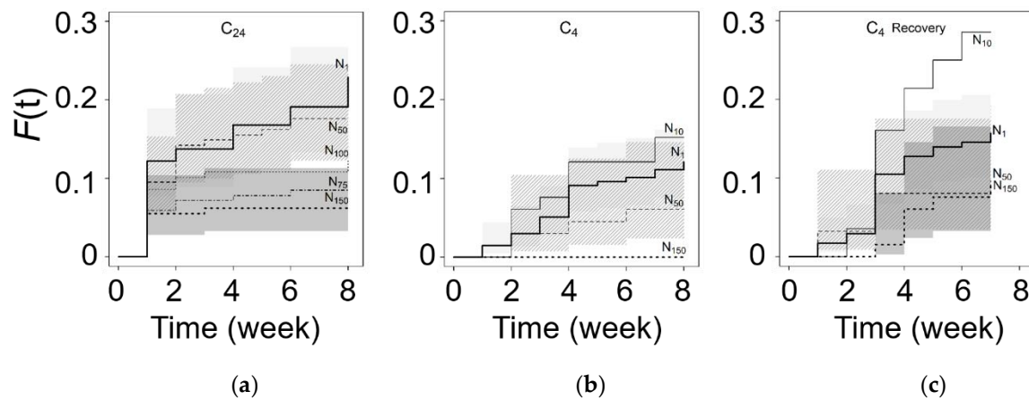
Figure 3. Cumulative germination probability, F(t) , with salinity ( N_x ; x = \text{NaCl} in mM) during germination (a, b) and recovery (c). Mean \pm 95% CI band for N_1 (light gray), N_{50} (diagonal stripes) and N_{150} (dark gray). Same symbols in all plots.
