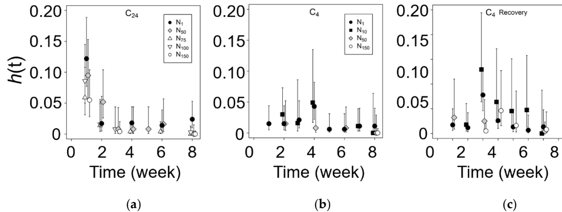
Figure 4. Hazard function, h(t) , with salinity during germination (a, b) and recovery (c). Mean \pm 95% CI bars. Same symbols in all graphs.
