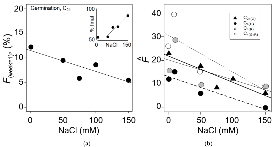
Figure 5. (a) Salinity and C 24 first-week germination probability, F_{(\text{week}=1)} ; y = -0.04^{ns}x + 11.5^{**} , r^2_{\text{adj}} = 0.633 , p > 0.067 , n = 5 . Inset: Salinity and relative germination risk for 1 st week relative to final germination (in percent), \% \text{ final} = 100 \cdot F_{(\text{week}=1)} / \hat{F} ; for 50-150 mM NaCl salinity range, y = 0.32^{**}x + 40.3^{**} , r^2_{\text{adj}} = 0.915 , p < 0.029 , n_{\text{obs}} = 4 . (b) Linear regression between salinity and \hat{F} in the trials (G = germination, R = recovery): solid bold , C 24(G) , r^2_{\text{adj}} = 0.77 , p < 0.031^{*} ; dashed , C 4 , r^2_{\text{adj}} = 0.76 , p < 0.034^{*} ; solid , C 4(R) , r^2_{\text{adj}} = 0.37 , p < 0.105^{ns} ; densely dashed , C 4(G+R) , r^2_{\text{adj}} = 0.47 , p < 0.197^{ns} .
