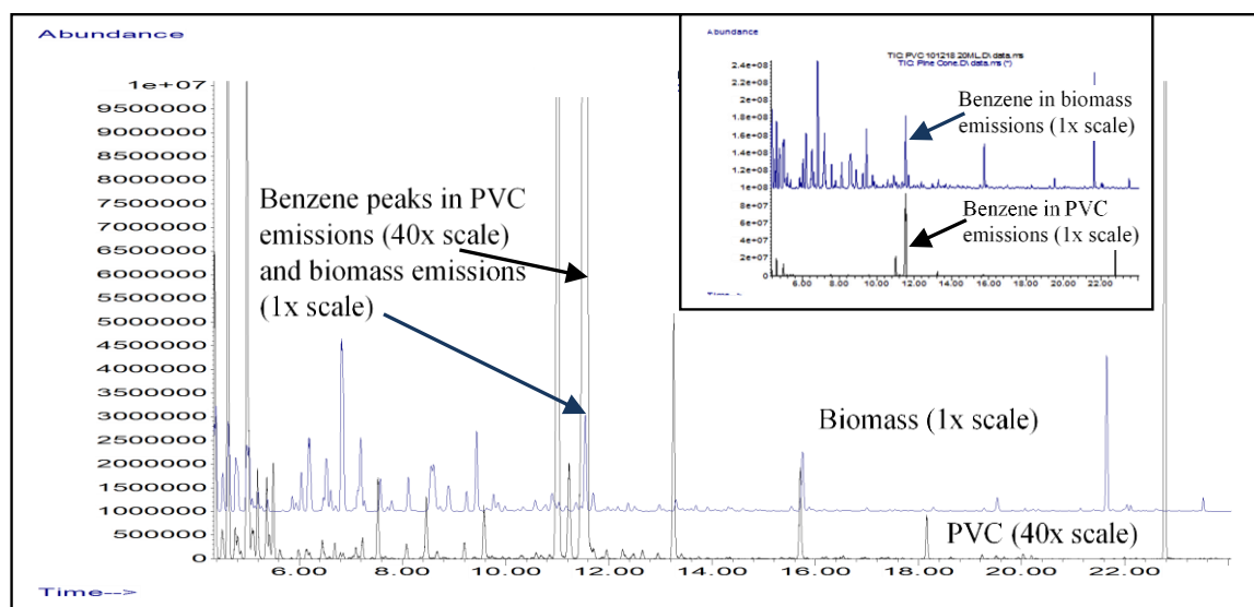
Figure 1. Overlaid GC-MS chromatograms of emissions from burning biomass compared to burning PVC pipes. Note that the scale for PVC emissions is expanded forty-fold to show the presence of about 85 VOCs detected at trace levels. The inset figure shows the same chromatograms on a common scale and the presence of about six major components in the burning PVC emissions.
