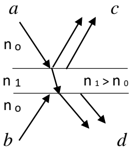
Fig. 1. A typical glass plate beam splitter. Photons arrive simultaneously at the upper dielectric boundary. n_1 > n_0
