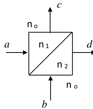
Fig. 2. A typical cubic prism beam splitter. Photons arrive simultaneously at the diagonal boundary interface. n_2 > n_1 > n_0
