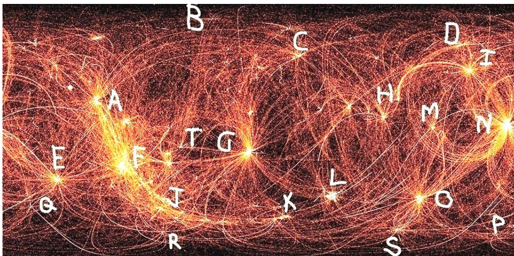
Figure 2: An X-ray map of the entire sky; posted originally by Universe.com [42]. Credit: NASA-NICER EXPT. (letters scripted on the original, color online).
