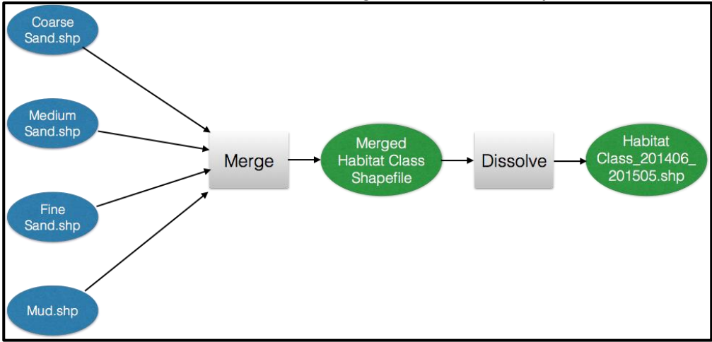
Figure 5. Flow-chart of data processing steps for manually segmented side-scan sonar - sediment classification into a habitat map for Assateague Island National Seashore, developed by the University of Delaware 2014-2015.
