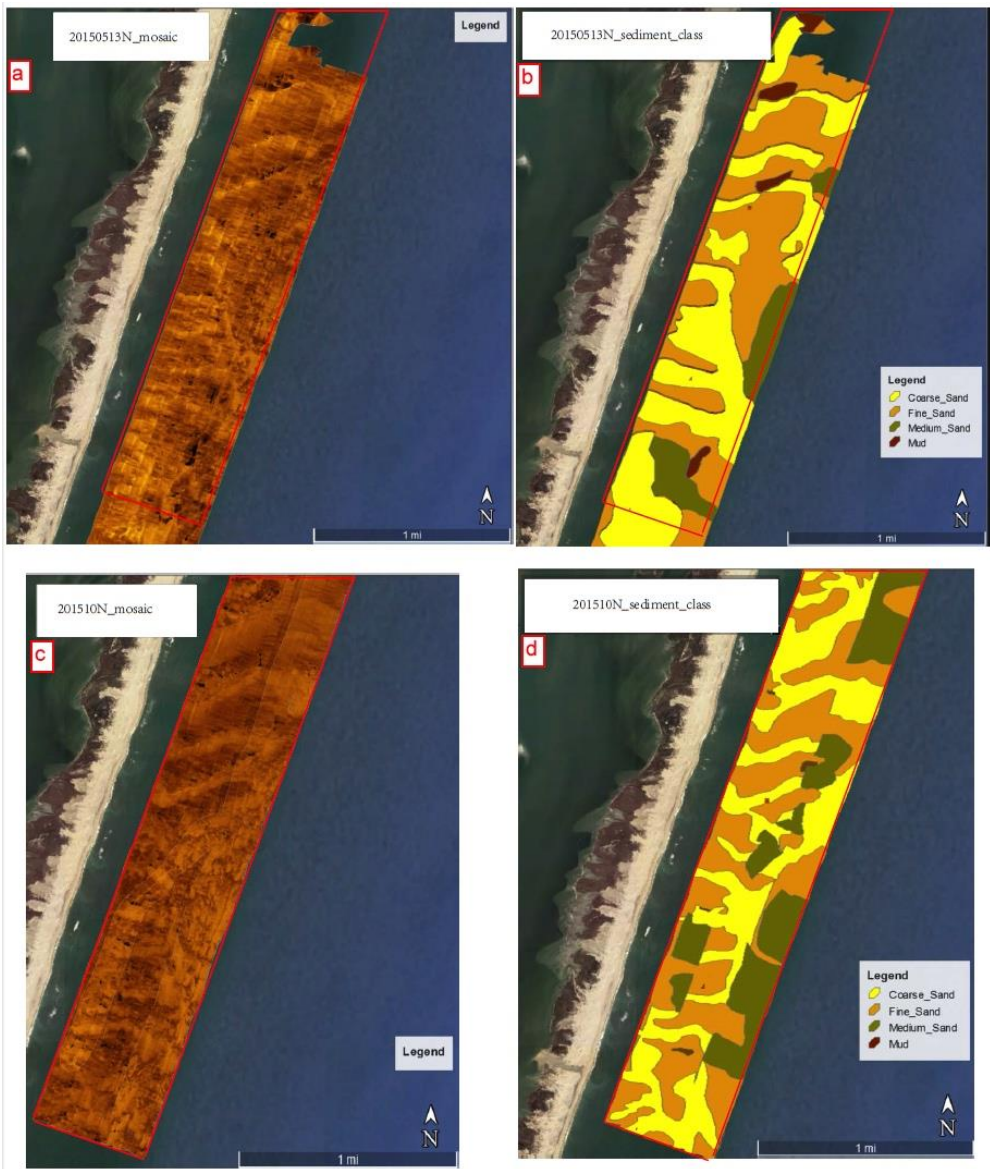
Figure 14: Side-scan sonar mosaic interpretation, Assateague Island National Seashore, Maryland (A) Side-scan sonar mosaics collected during May 13, 2015; (B) Interpretation of side-scan sonar data collected in May 13, 2015; (C) Side-scan sonar mosaics collected in October 2015; (D) Interpretation of side-scan sonar mosaics collected in October 2015. Note that red polygons represent the same areas mapped during both May 13, 2015 and October 2015.
