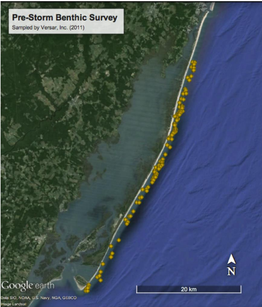
Figure 1. Pre-Sandy (2011) survey sites (n=125) sampled in October 2011 on the beach (n=15) and subtidally up to 1 km offshore (n=110) of Assateague Island National Seashore, Maryland. Image taken from Google Earth Pro Landsat, 2016.
