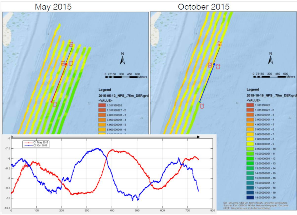
Figure 22. Bathymetry profile change after Hurricane Joaquin, Assateague Island National Seashore, Maryland. Red curved line represents the bathymetry profile C1 in May 2015 and blue curved line represents the bathymetry profile C2 in October 2015. Please note the Southwestward lateral shift of sand bars in the bathymetry profile. Inset scale is in meters on both axes.
