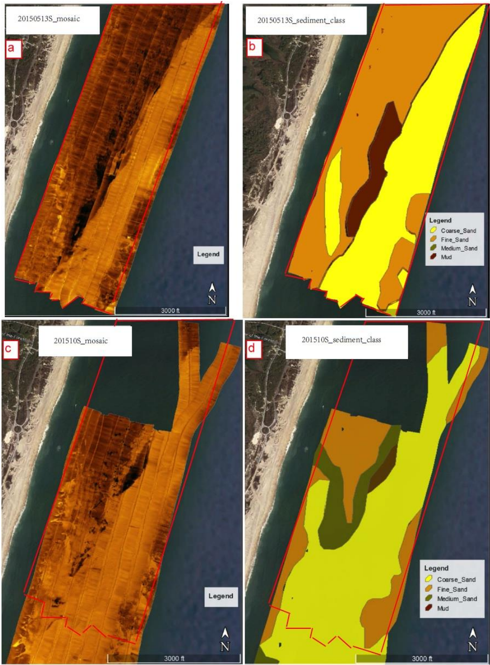
Figure 16: Side-scan sonar mosaic interpretation, Assateague Island National Seashore, Maryland. (A) Side-scan sonar mosaics collected during May 13, 2015; (B) Interpretation of side-scan sonar data collected in May 13, 2015; (C) side-scan sonar mosaics collected in October 2015; (D) Interpretation of side-scan sonar mosaics collected in October 2015. Note that red polygons represent the same areas mapped during both May 13, 2015 and October 2015.
