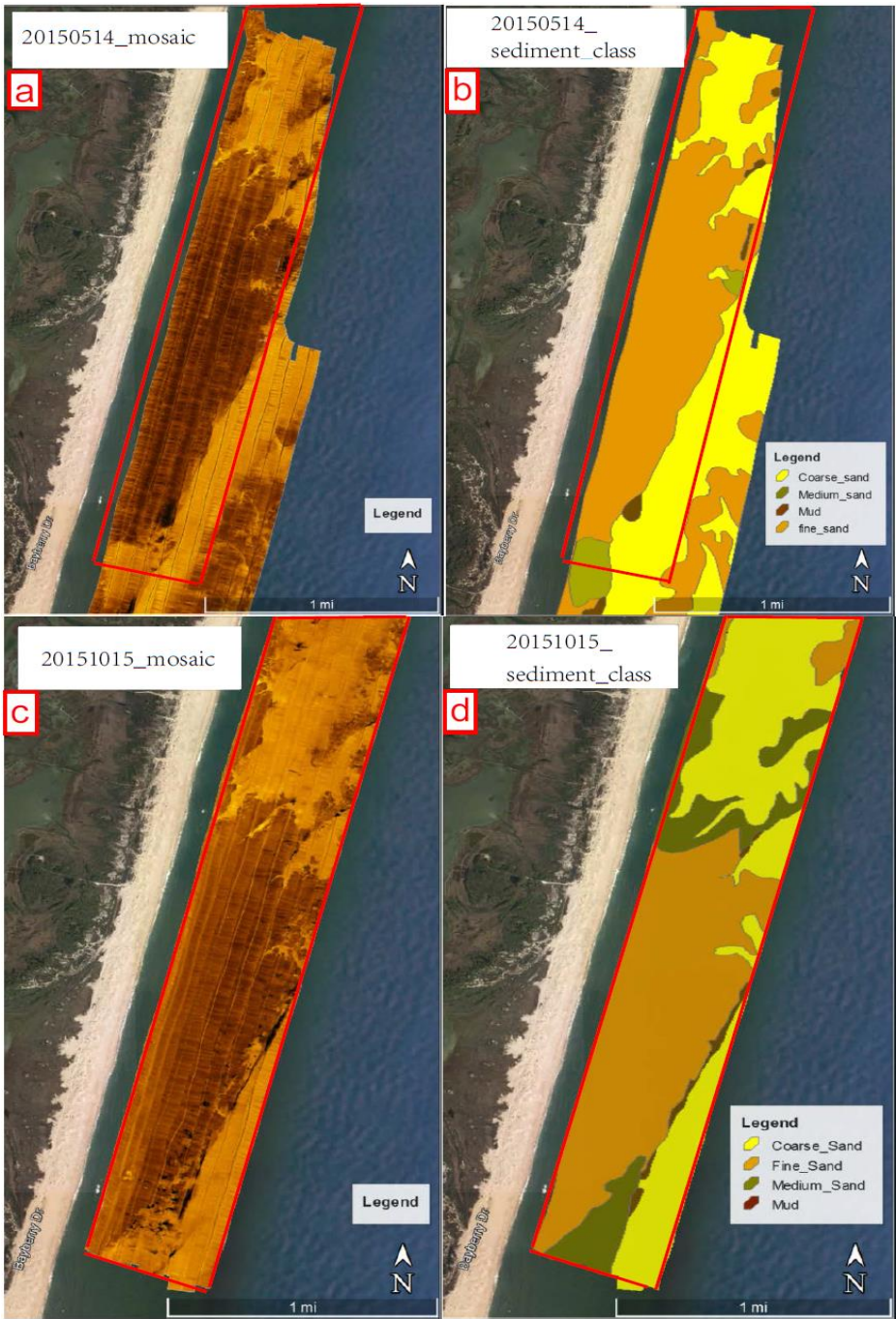
Figure 18: Side-scan sonar mosaic interpretation, Assateague Island National Seashore, Maryland. (A) Side-scan sonar mosaics collected during May 14, 2015; (B) Interpretation of side-scan sonar data collected in May 14, 2015; (C) Side-scan sonar mosaics collected in October 2015; (D) Interpretation of side-scan sonar mosaics collected in October 2015. Note that red polygons represent the same areas mapped during both May 14, 2015 and October 2015.
