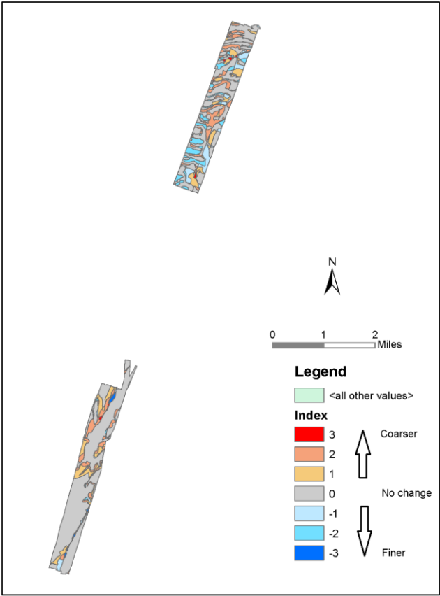
397 Figure 13. Sediment property change map for submerged resources of Assateague Island National 398 Seashore between May 2015 and October 2015. Positive sediment property change index means 399 seafloor became coarser, negative sediment property change index means seafloor became finer and 400 zero value means sediment texture did not change.
