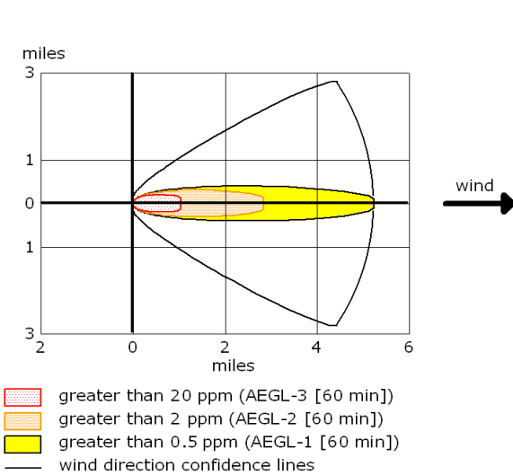
Figure 3: Simulation of high daily chlorine gas leakage from wells and water resources using ALOHA software
