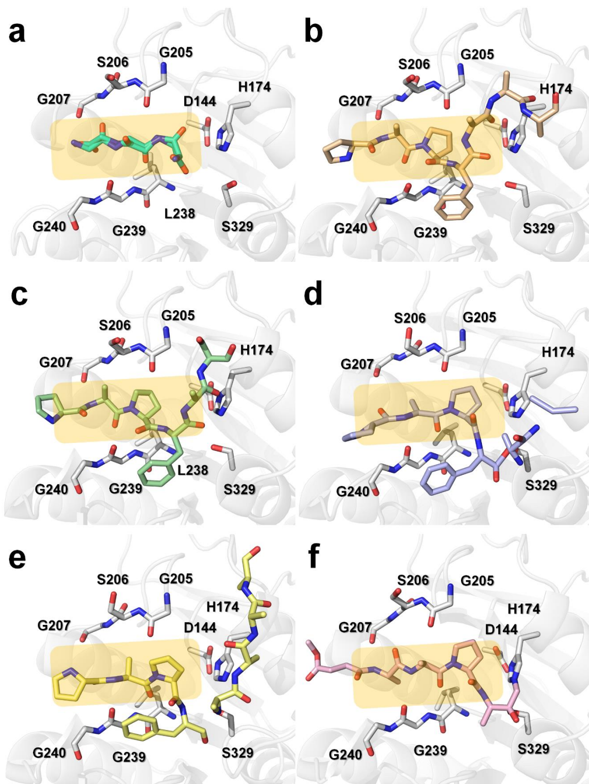
Figure S1. Comparison of substrate binding site of PaProK complexed with (a) triglycine or peptide based inhibitors from (b) PaProK-1P7V, (c) PaProK-1P7W, (d) PaProK-1PEK, (e) PaProK-1PFG and (f) PaProK-3PPK. The transparent box in orange indicates substrate binding site.
