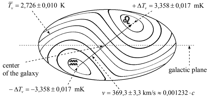
Fig. 6. Dipole anisotropy of cosmic microwave background shown in Hammer-Aitoff projection (own elaboration based on [7]).
