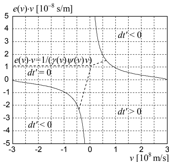
Fig. 11. Influence of parameter e(v) on time measurement in a mobile inertial system by an observer with universal frame of reference ( dt > 0 ).
