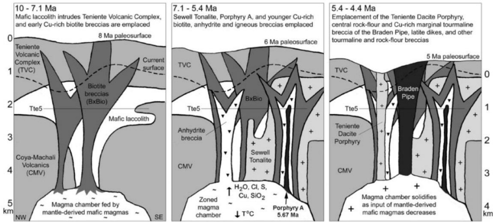
Figure 10. Model for the multistage development of the El Teniente deposit [23,32,33,39]. The main features of the model include (1) a large, long-lived ( \geq 3 \text{ Myr} ) open-system magma chamber, crystallizing at \geq 4 \text{ km} depth, fed from below by mantle-derived mafic magmas and exsolving mineral-rich high-temperature magmatic fluids through its roof to produce the large breccia pipes that are prominent features this deposit; (2) decreasing magma supply in the Late Miocene and Pliocene as subduction angle decreases, leading to crystallization and solidification of this chamber; (3) progressive uplift and erosion that enhances this crystallization and solidification process and results in telescoping of different types of breccia and igneous rocks [12,13]; (4) progressive igneous differentiation of the magma chamber associated with crystallization and volatile loss, generating felsic porphyries that intrude previously mineralized rocks above the chamber. No coeval volcanism is known to have occurred during mineralization, but once the chamber solidified, post-mineralization mantle-derived olivine lamprophyre dikes were emplaced.
