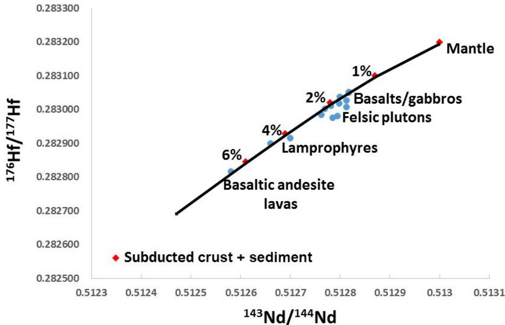
Figure 9. ^{176}\text{Hf}/^{177}\text{Hf} versus ^{143}\text{Nd}/^{144}\text{Nd} for samples from El Teniente (Table 2; blue circles) compared to isotopic values of a primitive mantle (Table 3) modified by the addition of various proportions (red diamonds) of subducted crust and sediment.
