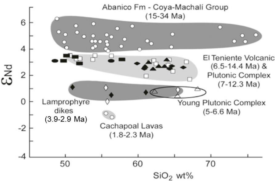
Figure 4. Published values of \epsilon_{\text{Nd}} vs \text{SiO}_2 (wt %) for igneous rocks of different ages from the transect across the Andes at the latitude of El Teniente ( 34^\circ\text{S} ; open symbols [10,14, 17,21-24]), compared with values for samples of the host-rocks in the deposit (filled symbols including the Teniente Mafic Complex (■), Sewell Tonalite (▲), felsic porphyries (◆), and Porphyry A granitoid (●); [23]). Although the youngest felsic plutons in the deposit are the same age (7.1 to 4.6 Ma) as rocks from the regionally defined Younger Plutonic Complex (6.6 to 5 Ma; [10]) they are isotopically similar to the older host-rocks of the deposit as well as to Teniente Volcanic and Plutonic Complex rocks.
