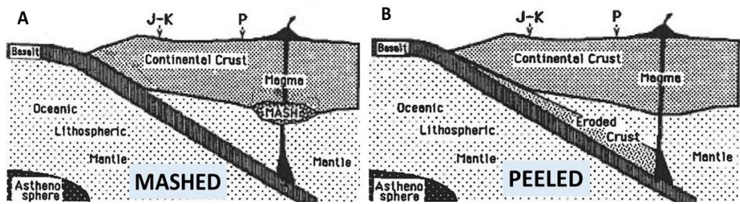
Figure 1. Two alternative explanations for the incorporation of continental crust into Andean magmas [1]. (A) MASHED on the left involves Mixing, Assimilation, Storage and Homogenization (MASH) at either the lower crust/mantle boundary or in the crust [2]. (B) PEELED on the right involves recycling of subduction eroded crust into the mantle wedge source [3-5]. J-K and P indicate the position of the Jurassic-Cretaceous and Pliocene plutonic belts, respectively, in the Andes of northern Chile. The recently active volcanic arc is ~250 km east of the Jurassic arc as a result of subduction erosion [6].
