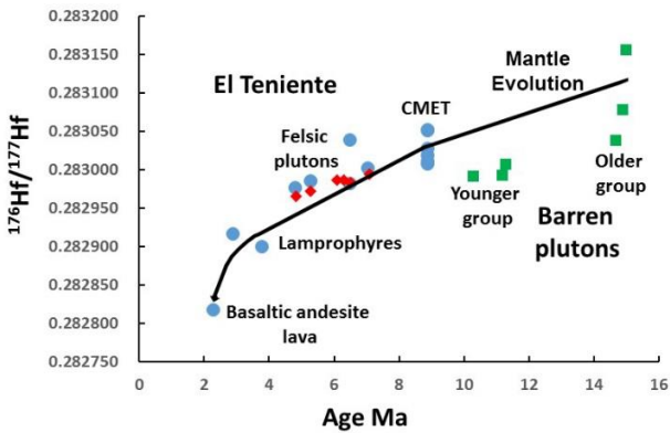
Figure 7. ^{176}\text{Hf}/^{177}\text{Hf} versus age (Ma) for samples from El Teniente (blue circles from Table 2; red diamonds from [37]) and Middle Miocene barren plutons in the same general area (green squares from [50]). Mantle isotopic evolution line is draw from average of older group of Middle Miocene barren plutons through Late Miocene Teniente Mafic Complex (CMET) olivine basalts and gabbros, to olivine lamprophyres and olivine-bearing basaltic andesites, ignoring the younger group of barren plutons because these have macroscopic evidence for intra-crustal assimilation [50]. The amount of subducted crust plus sediment added to the mantle to generate this line is indicated in Figure 9.
