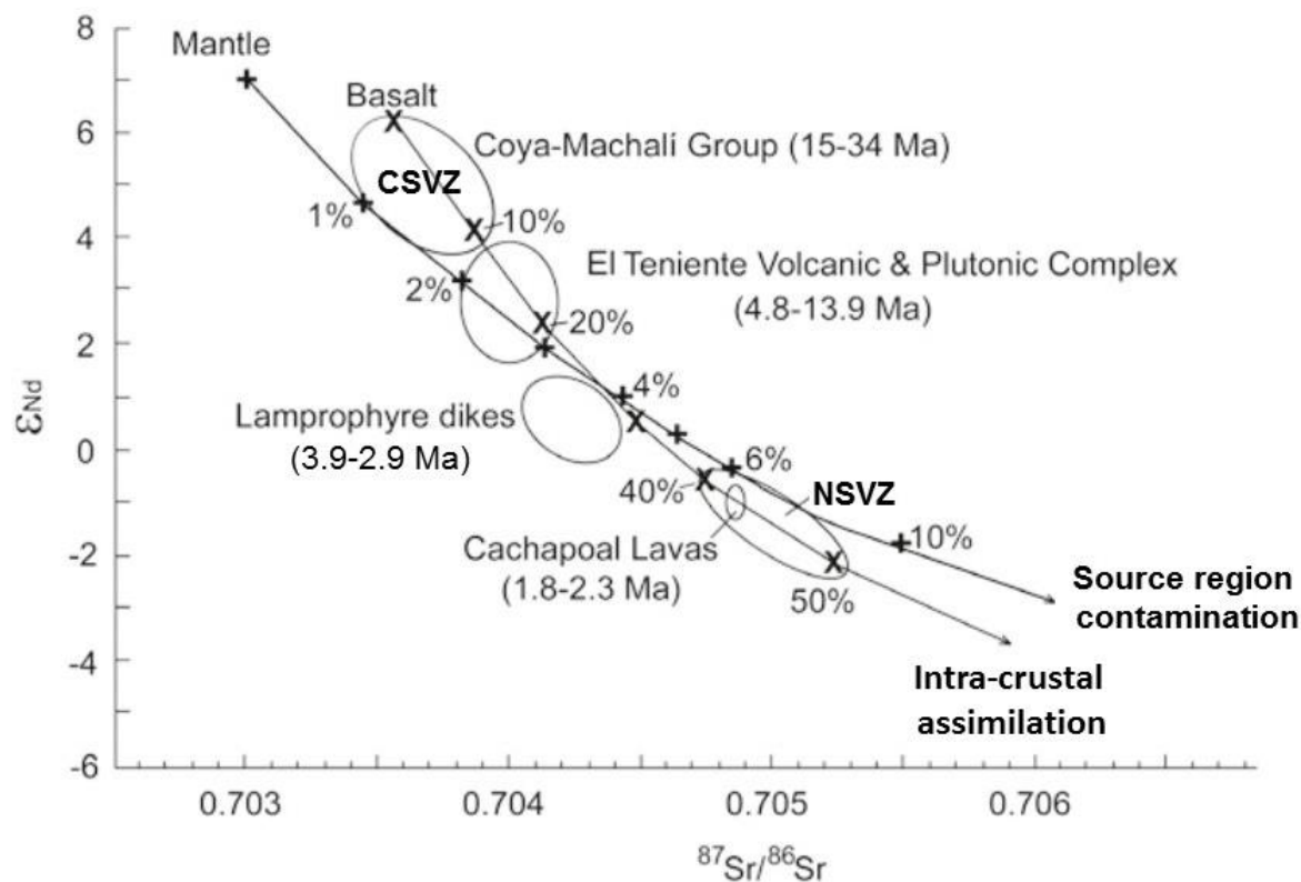
Figure 5. Sr versus Nd isotopic values of the various groups of igneous rocks of different ages across a transect of the Andes at the latitude of El Teniente (34°S; fields and data sources from Figure 4). The figure illustrates both a source region contamination model of primitive mantle ( \text{Sr}=36 ppm with ^{87}\text{Sr}/^{86}\text{Sr}=0.703 and \text{Nd}=1.8 ppm with \epsilon_{\text{Nd}}=+7 ; [21]) mixed with various proportion of subducted crust and sediment ( \text{Sr}=380 ppm with ^{87}\text{Sr}/^{86}\text{Sr}=0.70763 and \text{Nd}=42.3 ppm with \epsilon_{\text{Nd}}=-5.1 ), and also a MASH model for a Coya-Machali basalt ( \text{Sr}=450 ppm with ^{87}\text{Sr}/^{86}\text{Sr}=0.7035 and \text{Nd}=9 ppm with \epsilon_{\text{Nd}}=+6 ) assimilating various proportion of Paleozoic-Triassic Andean granite basement ( \text{Sr}=350 ppm with ^{87}\text{Sr}/^{86}\text{Sr}=0.7075 and \text{Nd}=20 ppm with \epsilon_{\text{Nd}}=-6 ; [10]) Both models reproduce the isotopic compositions of the progressively younger rocks in the transect, but the latter model requires assimilation of unacceptably high proportions of granite crust and is inconsistent with generation of primitive low \text{SiO}_2 olivine-bearing mafic rocks in each age group, as well as the increasingly higher Sr content of the progressively younger rocks, which is due instead to decreasing degrees of partial mantle melting [3-5,10], consistent with decreasing volume of magmas erupted through time at this latitude in the Andes.
